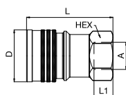
Female Thread
