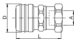
Female Thread
