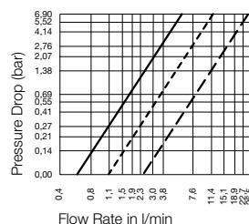
Flow Capacity with Water
