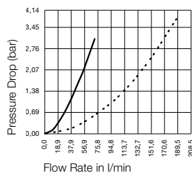
Flow Capacity with Hydraulic Oil with Viscosity of 30cSt
