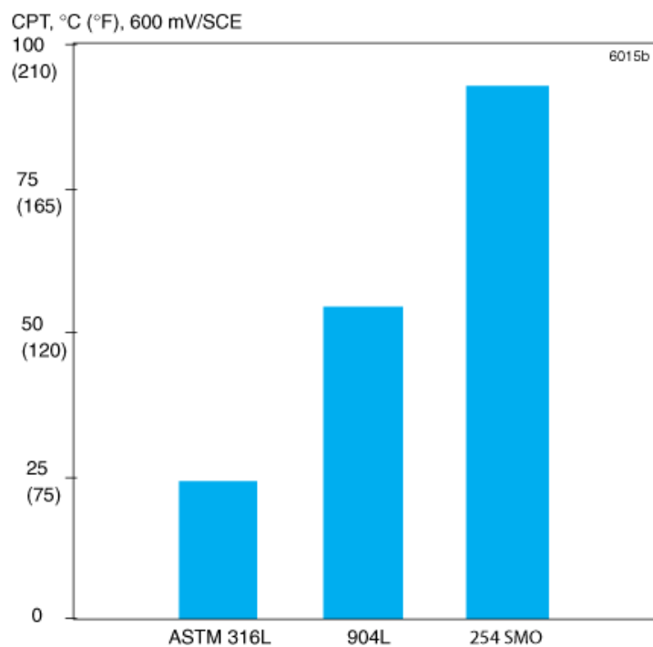
Figure 3. Critical pitting temperature (CPT) in 3% NaCl, 600 mV/SCE.
