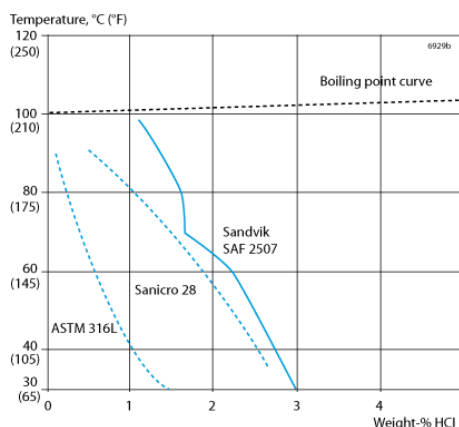
Figure 9. Isocorrosion diagram in hydrochloric acid. The curves represent a corrosion rate of 0.1 mm/year (4 mpy) in stagnant test solution.
