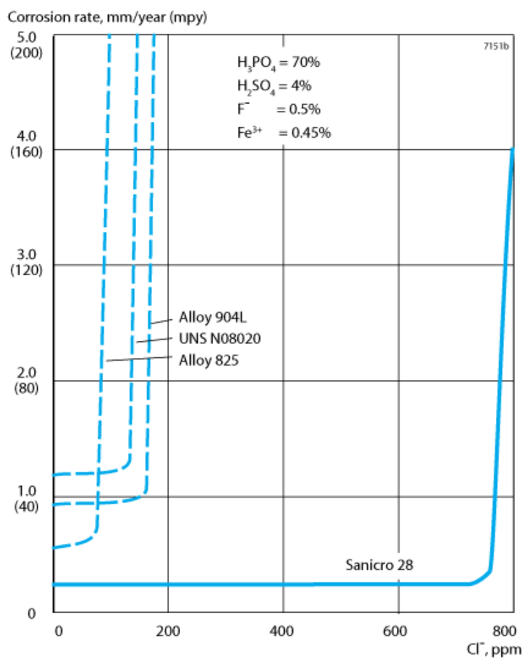
Figure 1. Corrosion rate in contaminated phosphoric acid at different chloride concentrations 100°C (210°F). Comparison of Sanicro® 28 and other alloys (chemical compositions given in table 1).
