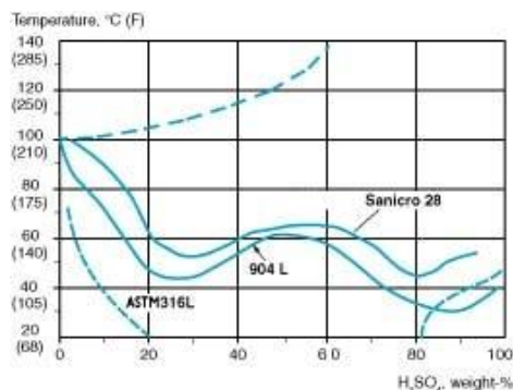
Figure 3. Isocorrosion diagram for Sanicro® 28, Alloy 904L and ASTM 316L, in deaerated sulfuric acid. The curves
