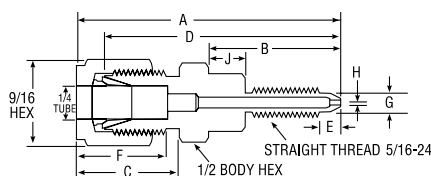
Calibration Adapter for Rosemount/Foxboro DP Transmitters
