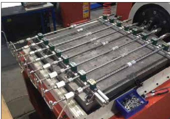
Vibration test
