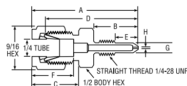
Calibration Adapter for Honeywell DP Transmitters
