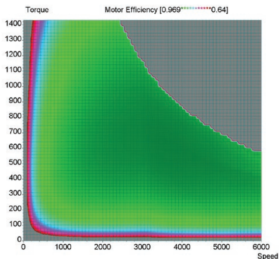
GVM310-250-BA-2 in motor operation mode
