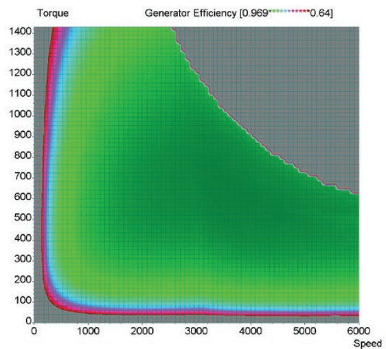
GVM310-250-BA-2 in generator operation mode
