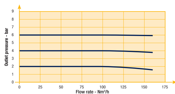
Flow Curve 1"
