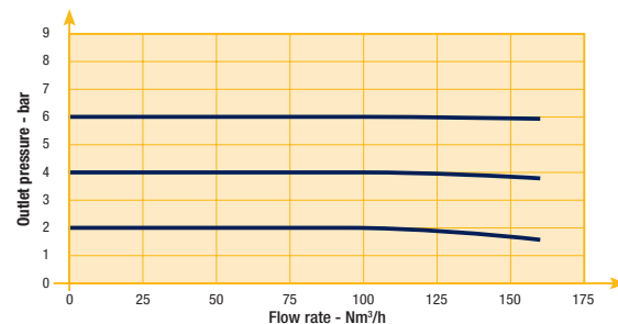
Flow Curve 1"
