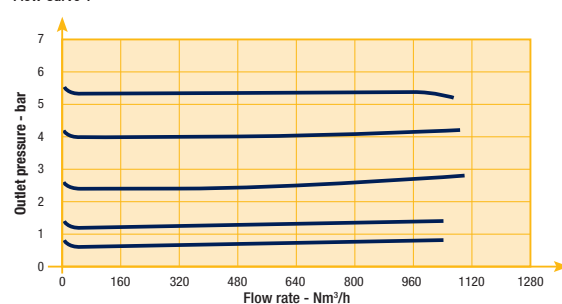
Flow Curve 2"
