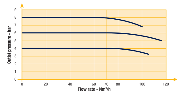
Flow Curve Basic 1/4"
