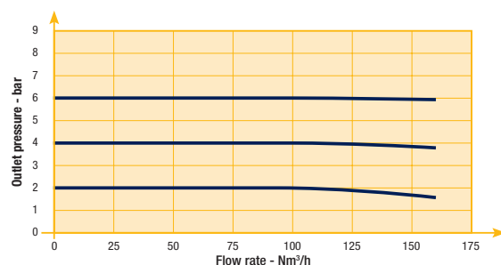
Flow Curve 1/2"
