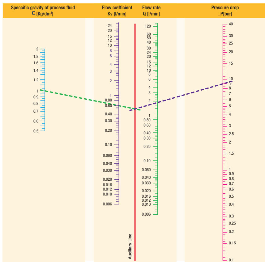
Monogram for liquid flow calculation
