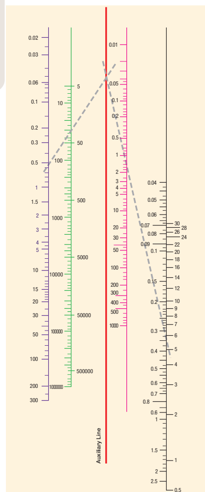
Diagram 3 for Dry Saturated Steam
