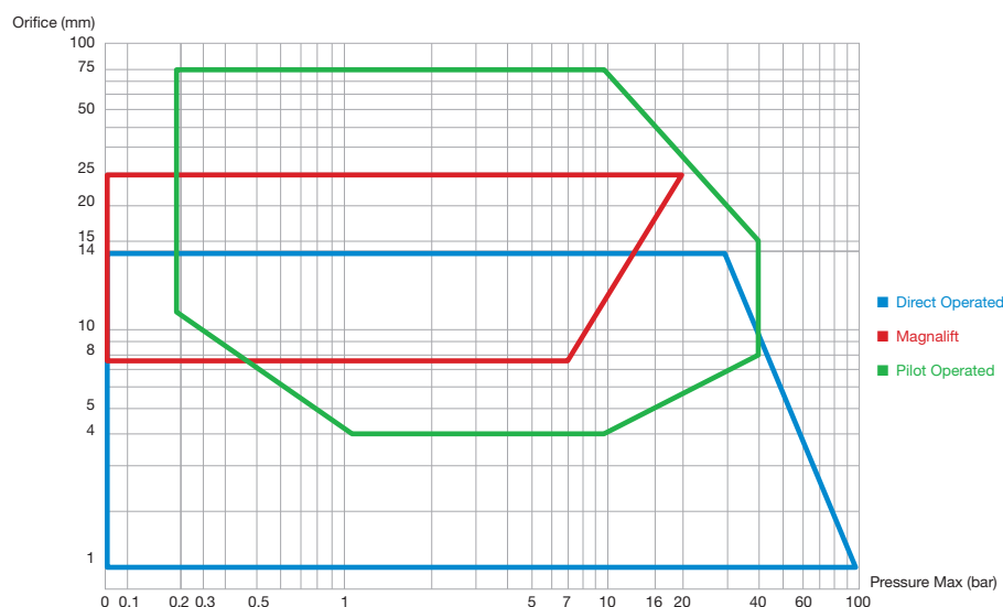
Areas of operation of Parker solenoid valves.
