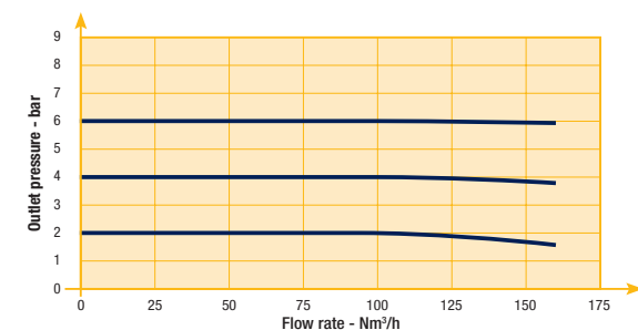
Flow Curve Basic 1/2"
