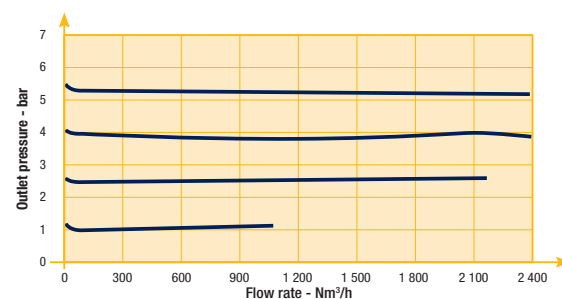
Flow Curve 2"
