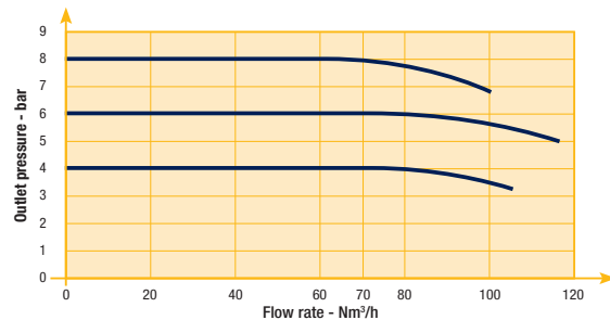
Flow Curve 1/4"
