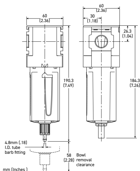
Manual Drain
