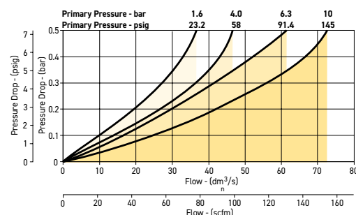
P33FA 3/4" Filter
