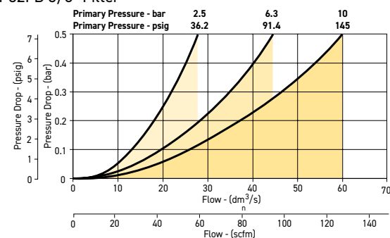
P32FB 3/8" Filter
