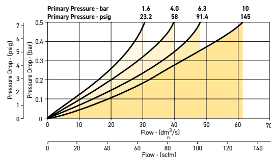
P33FA 1/2" Filter
