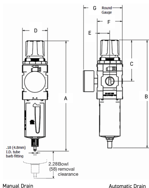
Manual Drain
