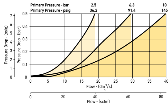
P32FB 1/4" Filter
