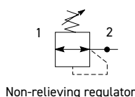
Non-relieving regulator
