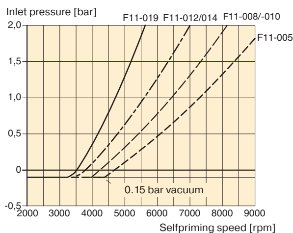
Diagram 2. Min required inlet pressure for Pump.
