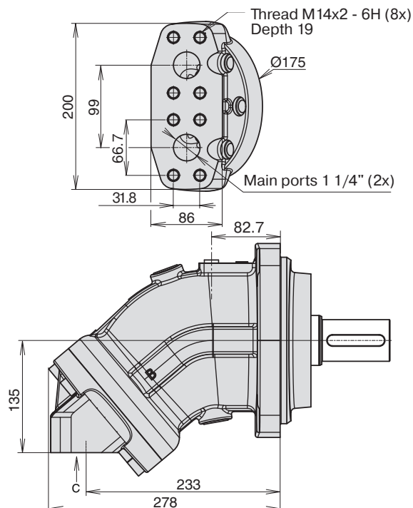
Main ports type D (90 deg Horizontal)
