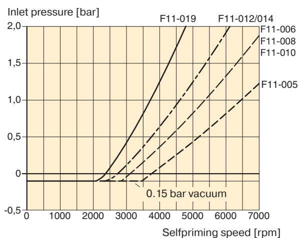
Diagram 1. Min required inlet pressure for Motor.
