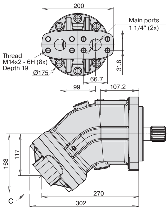
Main ports type K (40 deg rear)
