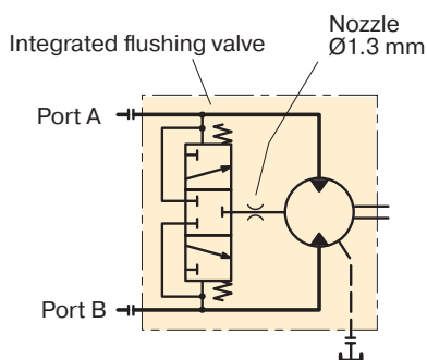
Hydraulic schematic.
