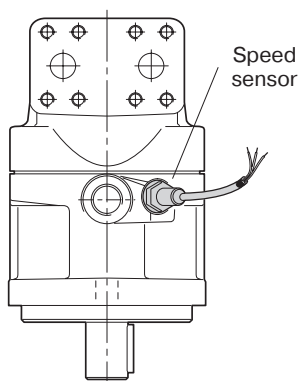
F10/F12 with speed sensor.
