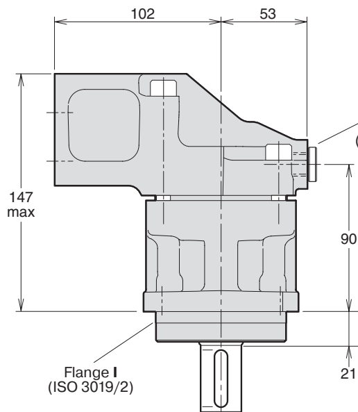
Drain port D M16x1.5 (depth 12; ISO 9974-1)
