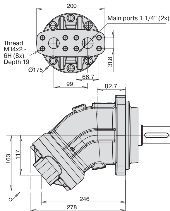
Main ports type K (40 deg rear)
