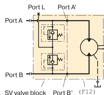
Hydraulic schematic.
