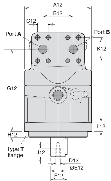
Shown: F12-60 with 2 bolt flange
