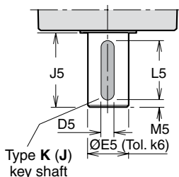
Shaft option K (J)
