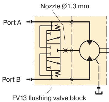
Hydraulic schematic.
