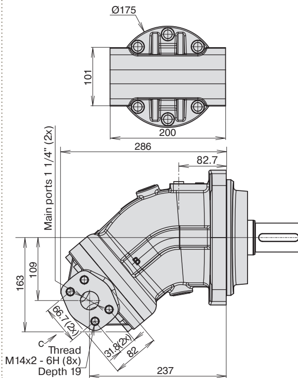
Main ports type M (Side ports)
