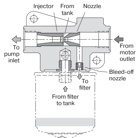
BLA boost unit cross section.
