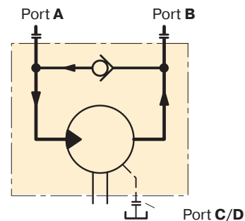
Schematic Fan motor with anti cavitation valve
