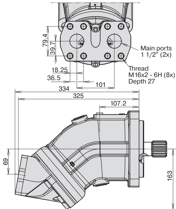
Main ports type A (180 deg Vertical)
