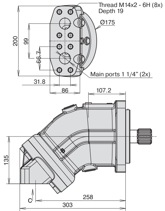
Main ports type D (90 deg Horizontal)
