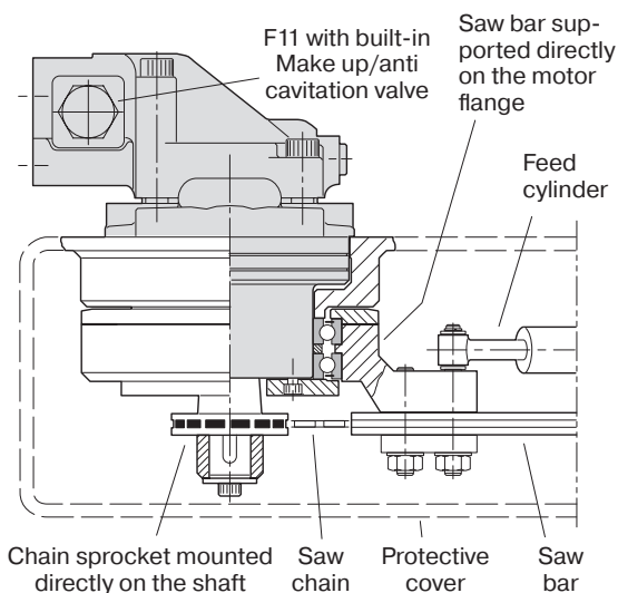
Chain saw installation (example; F11-10 shown)
