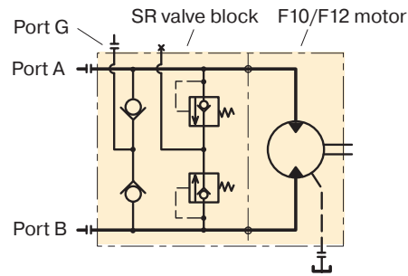
SR valve block schematic.
