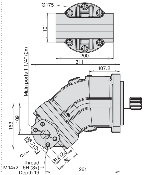
Main ports type M (Side ports)
