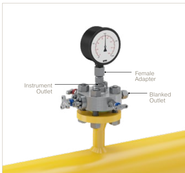
Monoflange with a dual outlet option mounted directly to a horizontal pipe.
