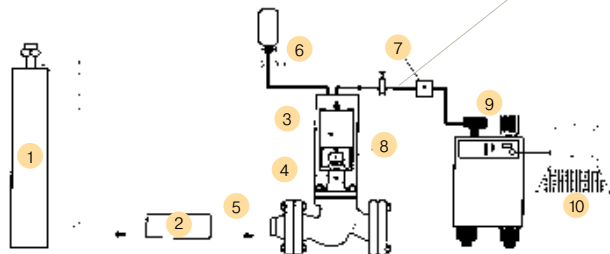
Prototype testing schematic as per ISO 15848-1
