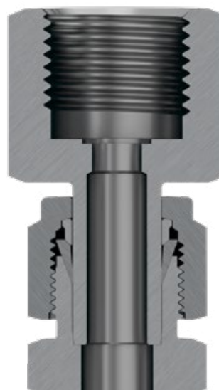
Parker's tube end female adapter installed into an A-LOK® outlet connection.
