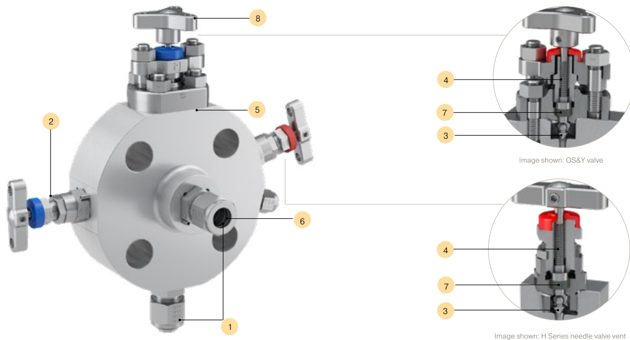
Monoflange with Outside Screw & Yoke (OS&Y) valve primary isolation
