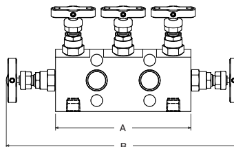
Example shown: 5-valve extruded direct mount manifold with Parker Superior Advantage fully integrated inverted A-LOK® tube fitting connections.
