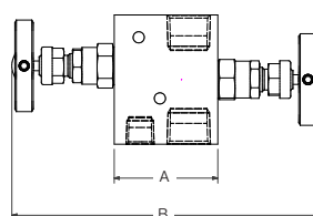
Example shown: 2-valve manifold with integral A-LOK® connections.
