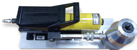
Parker Part No. MPI AIR PUMP KIT
