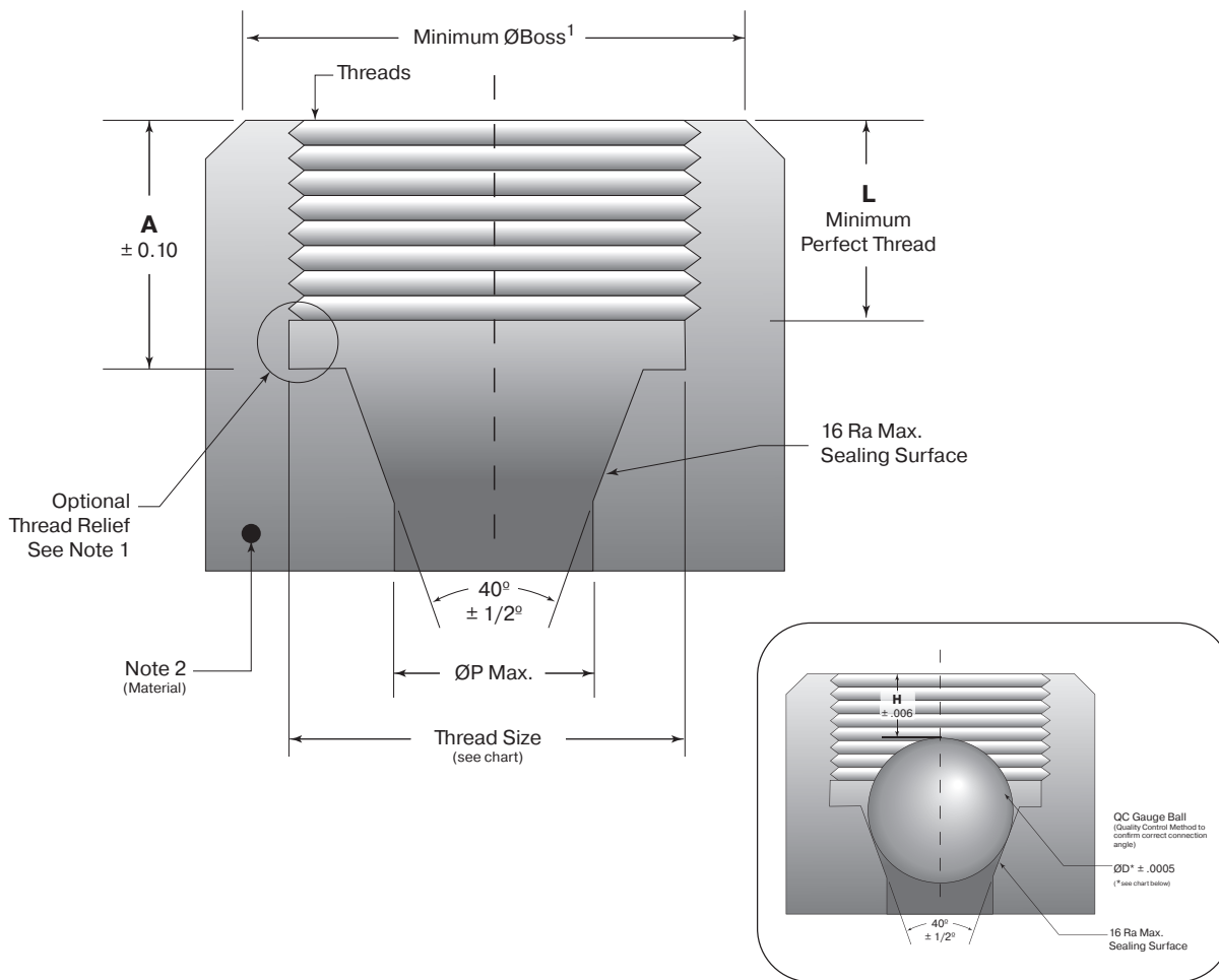
Figure 2 (Shown with QC Gauge Ball in-place)
