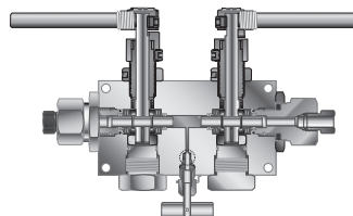
MADBB Series Double Block & Bleed Ball Valve
