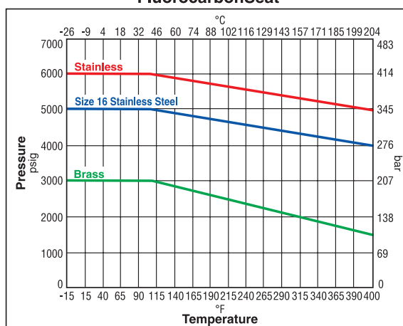
Fluorocarbon Seat
