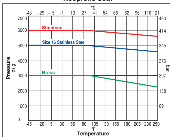
Neoprene Seat
