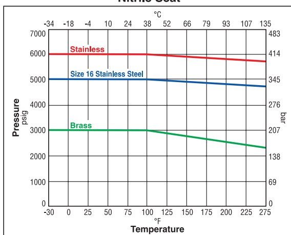
Nitrile Seat
