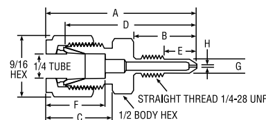
Calibration Adapter for Honeywell DP Transmitters
