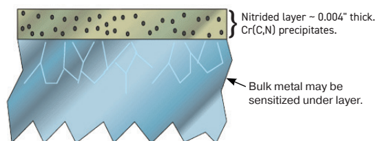
Conventional gas nitrided stainless steel
