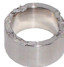
As-machined Test Piece After Ferric Chloride Test
