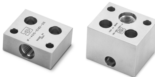
End Access
