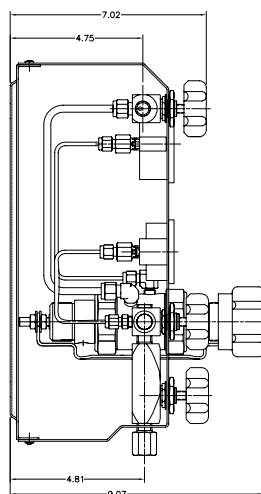
Without Outlet Regulator
