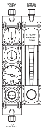
Basic Fast Loop System
