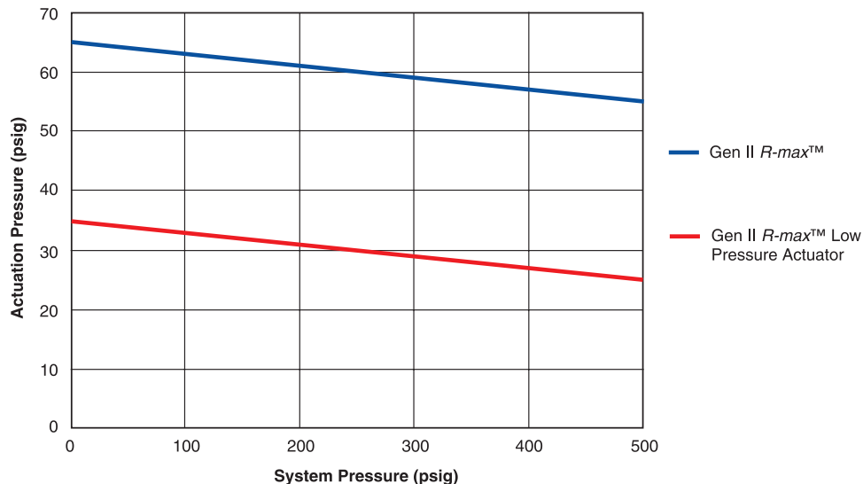
Actuation Pressure vs System Pressure
