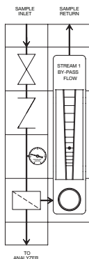
Basic Fast Loop System
