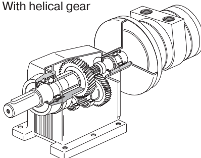
With helical gear
