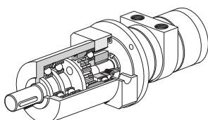
With planetary gear
