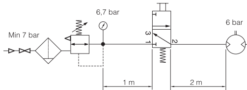
Shut-off, filtering, pressure regulation and control valve
