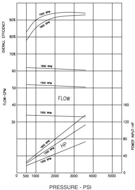
Performance curves Series 8 Pump at full displacement
