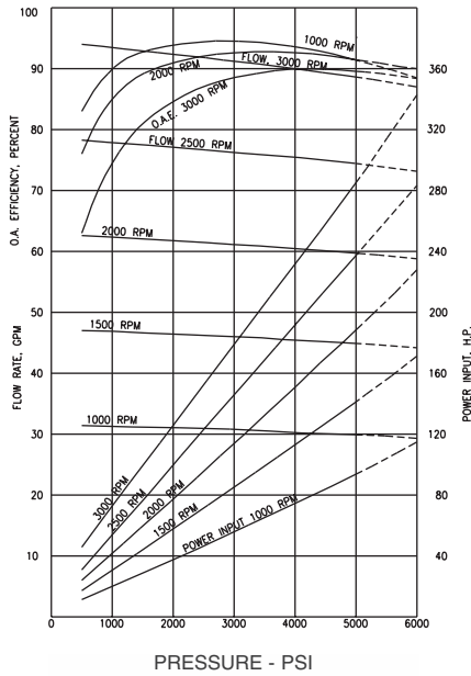
Performance curves Series 7 Pump at full displacement
