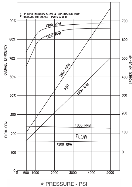
Performance curves Series 30 Pump at full displacement
