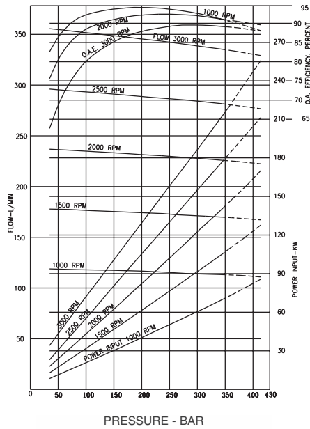
Performance curves Series 7 Pump at full displacement
