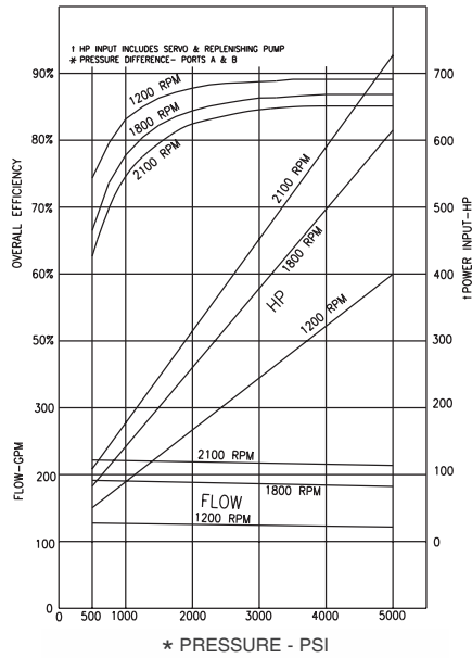
Performance curves Series 24 Pump at full displacement
