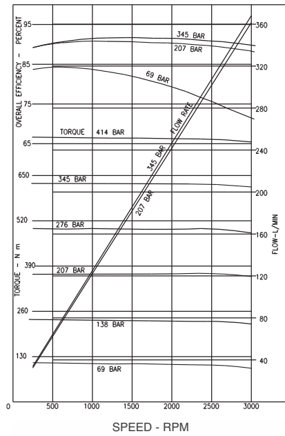
Performance curves Series 7 Motor at full displacement
