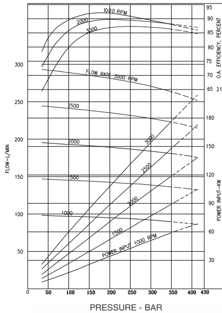
Performance curves Series 6 Pump at full displacement
