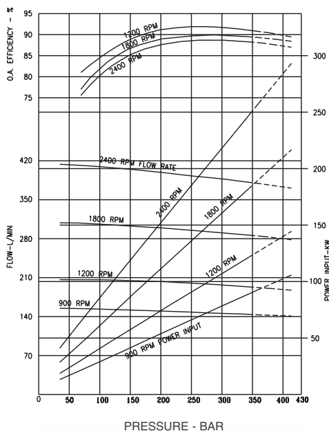
Performance curves Series 11 Pump at full displacement
