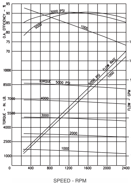
Performance curves Series 11 Motor at full displacement
