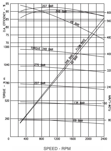
Performance curves Series 14 Motor at full displacement
