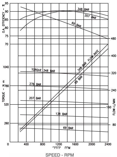
Performance curves Series 11 Motor at full displacement
