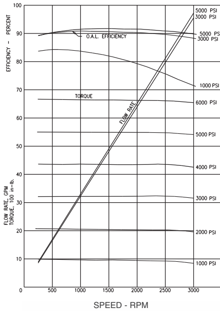
Performance curves Series 7 Motor at full displacement
