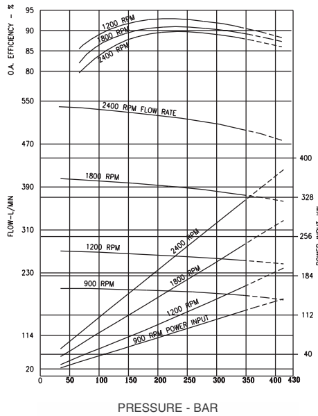
Performance curves Series 14 Pump at full displacement
