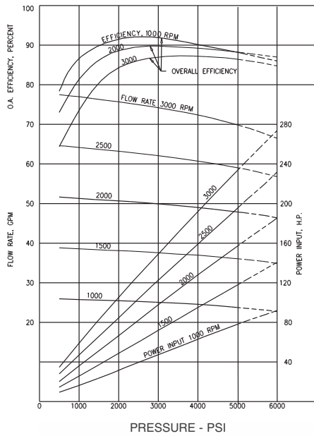
Performance curves Series 6 Pump at full displacement
