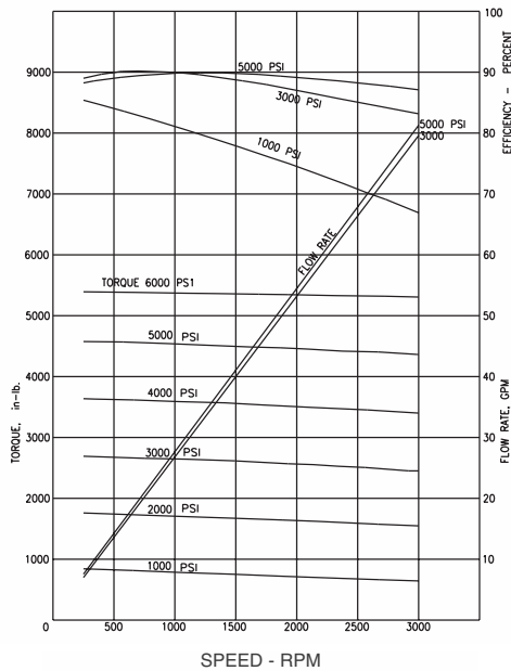
Performance curves Series 6 Motor at full displacement
