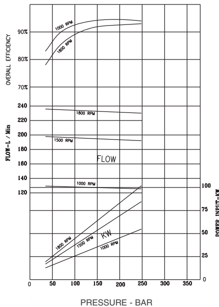
Performance curves Series 8 Pump at full displacement
