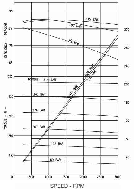
Performance curves Series 6 Motor at full displacement
