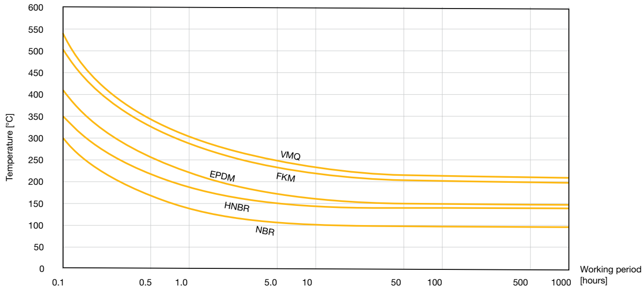
Fig. 7.1 High temperature limitations for various elastomeric materials
