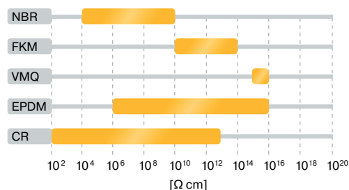
Fig. 8.9 Specific electrical resistance
