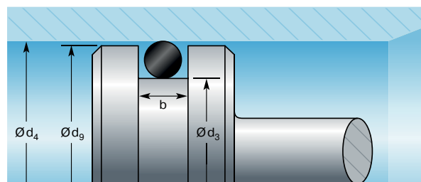
Fig. 3.9 Piston seal – radial compression
