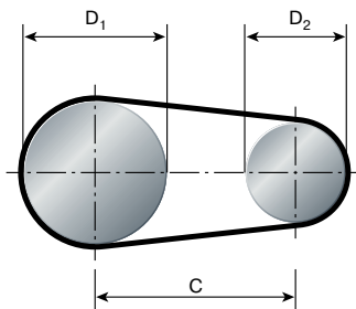
Fig. 2.19 Open design
