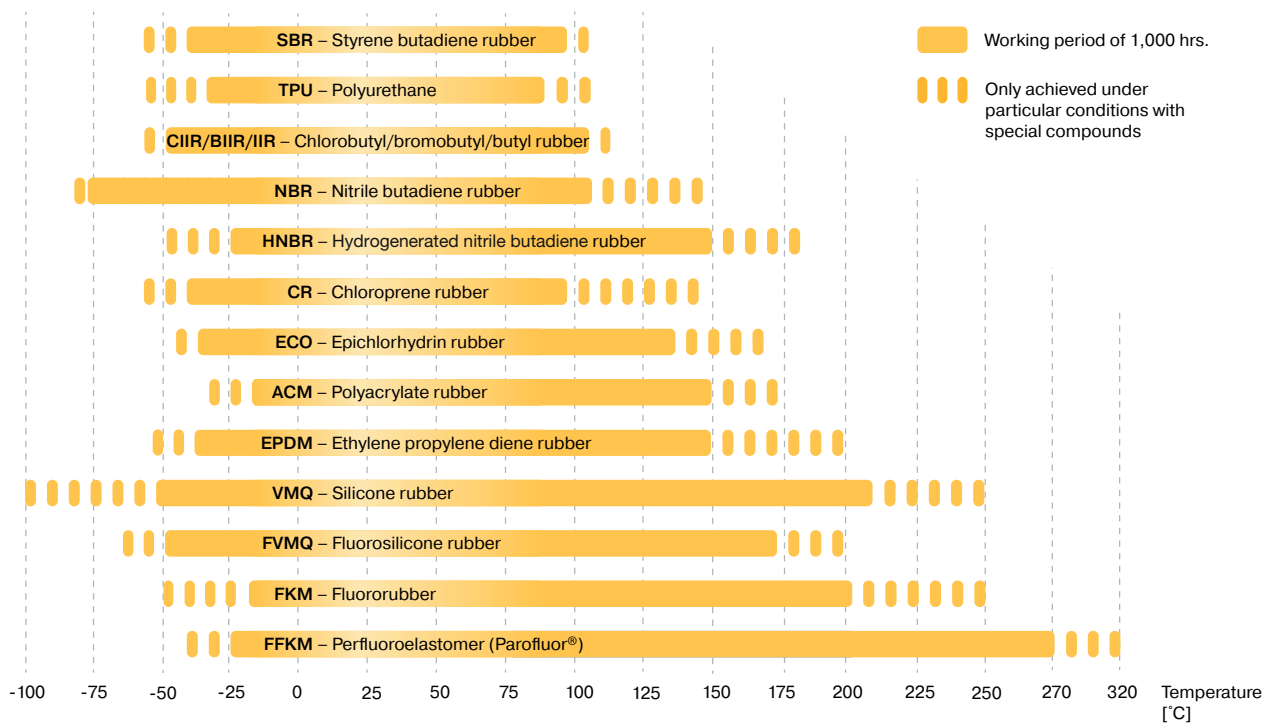
Fig. 6.4 High-temperature limits for various elastomeric materials
