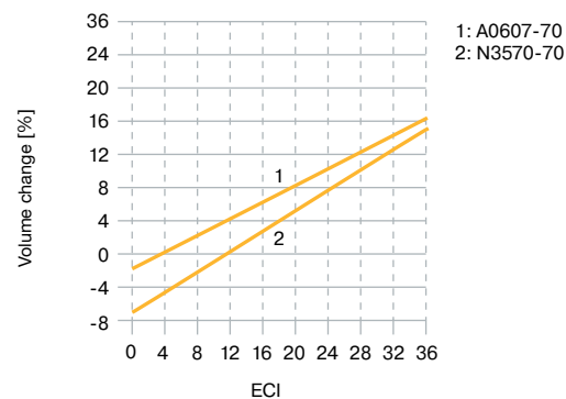
Fig. 8.7 Swelling characteristics of Parker compounds
