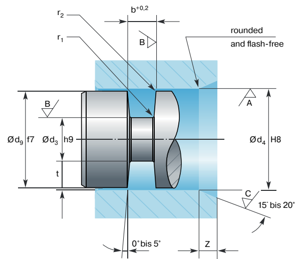
Fig. 2.15 Piston seal – hydraulic and pneumatic
