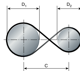
Fig. 2.20 Crossed design
