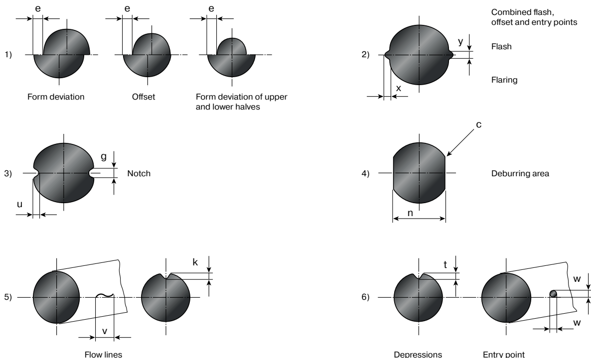
Fig. 9.1 Mould and surface finish defects
