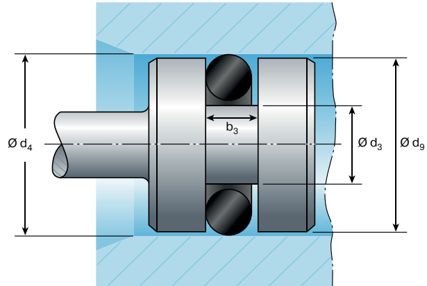
Fig. 3.15 Floating design – no deformation
