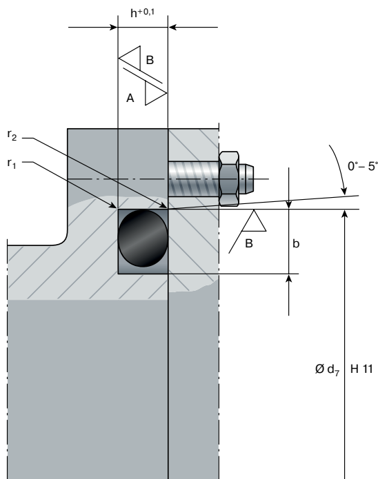
Fig. 2.8 Pressure from inside
