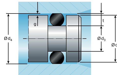
Fig. 8.34 With perfect concentricity
