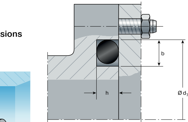
Fig. 3.3 Flange seal – axial compression
