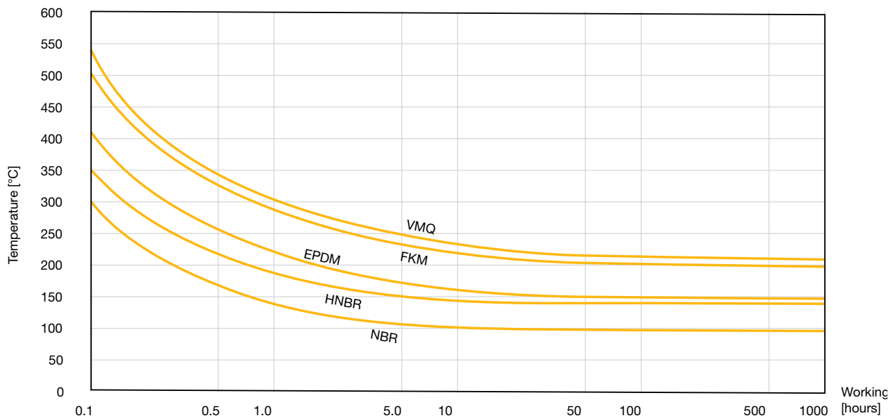
Fig. 6.5 High-temperature limits for various elastomeric materials
