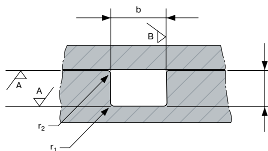
Fig. 7.6 Dimensions of vacuum gland, static application
