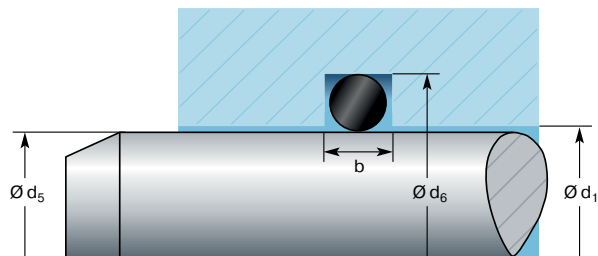
Fig. 3.10 Rod seal – radial compression
