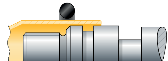
Fig. 2.29 Use of a fitting aid
