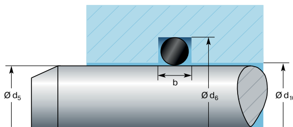
Fig. 3.2 Rod seal – radial compression
