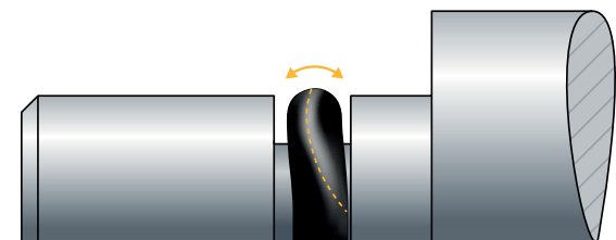
Fig. 2.28 O-Ring fitted rolled
