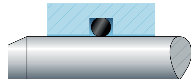
Fig. 2.1 Female gland ("rod seal"): O-Ring with radial compression
