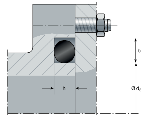
Fig. 3.4 Flange seal – axial deformation
