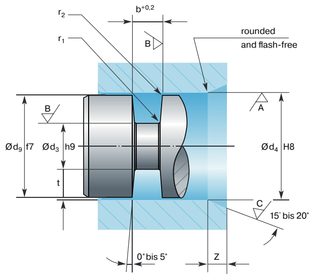
Fig. 2.5 Gland in inside element
