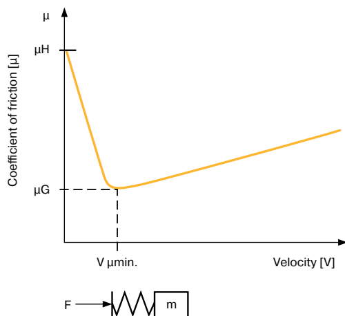
Fig. 8.21 System diagram for stick-slip effect
