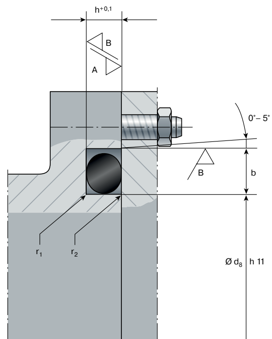
Fig. 2.9 Pressure from outside
