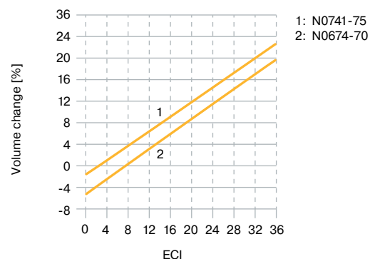
Fig. 8.8 Swelling characteristics of Parker compounds
