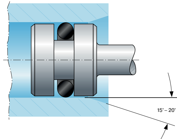
Fig. 2.22 Assembly example of piston
