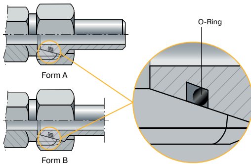
Fig. 4.4 Assembly
