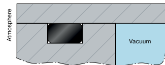
Fig. 7.5 Vacuum O-Ring gland
