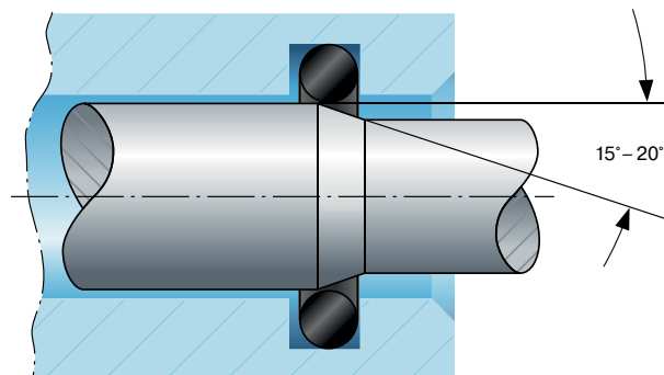
Fig. 2.23 Assembly example of rod
