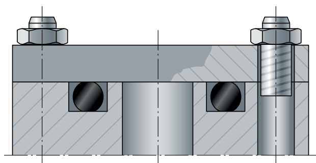
Fig. 2.3 Face seal: O-Ring deformed axially
