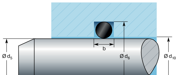
Fig. 3.14 Rod seal – radial compression
