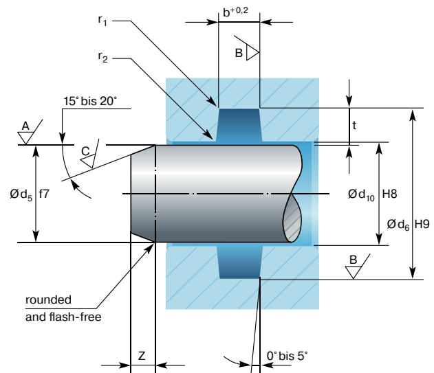
Fig. 2.6 Gland in outside element
