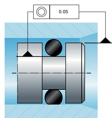
Fig. 8.36 With maximum eccentricity and non-concentric piston and groove diameters
