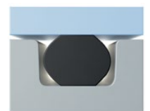
Fig. 10.1 Due to its elastic behaviour the O-ring exerts its sealing effect in the compressed, non-pressurised state between two sealing areas.
