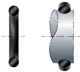
Fig. 8.12 Left: unstretched O-Ring, right: stretched O-Ring
