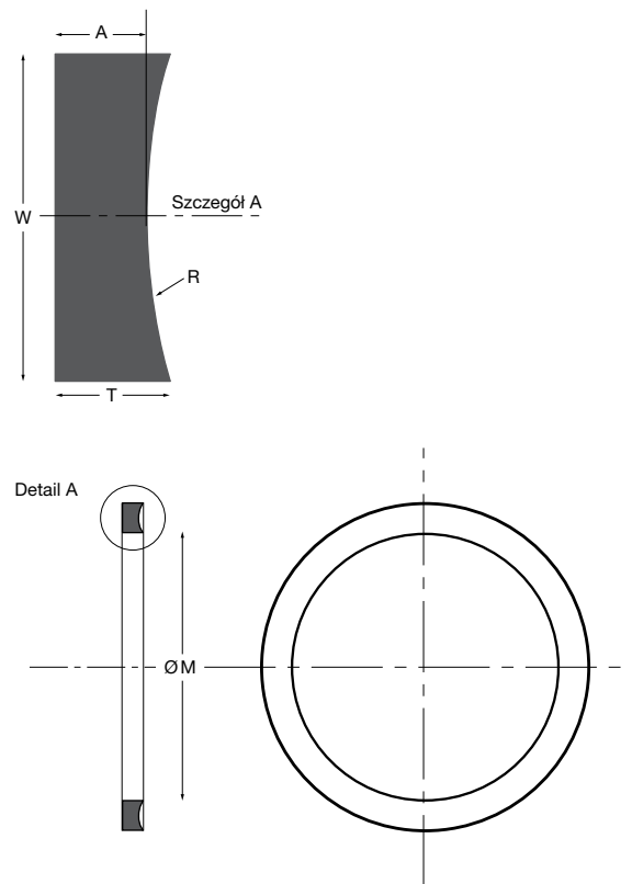
Fig. 4.11 Parbak® back-up ring
