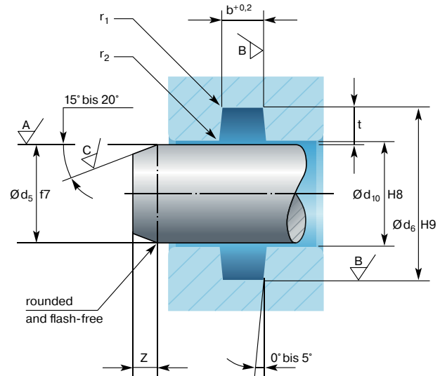
Fig. 2.14 Rod seal – hydraulic and pneumatic
