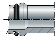
Fig. 4.3 Threaded fitting with 24° conical seal face: form B for hose connector
