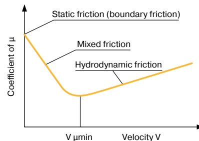
Fig. 8.18 Stribeck curve
