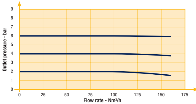
Flow Curve 1/2"
