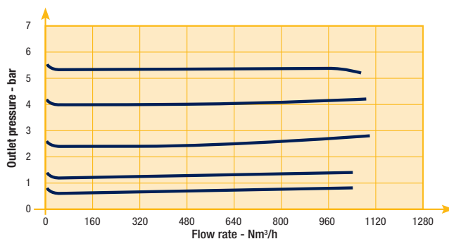
Flow Curve 2"
