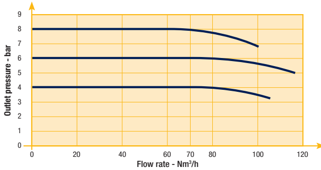
Flow Curve 1/4"
