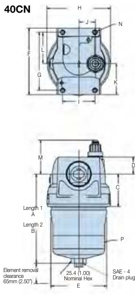
Dimensions in mm (inch)
