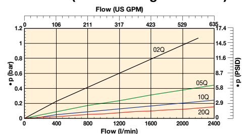
IN2400 (Element length code 18)
