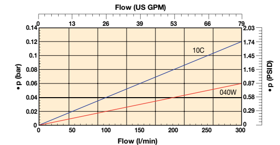
STF230 (Element length code 7)
