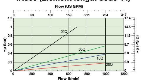
IN1500 (Element length code 16)
