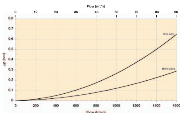
Length 1 elements/one side
