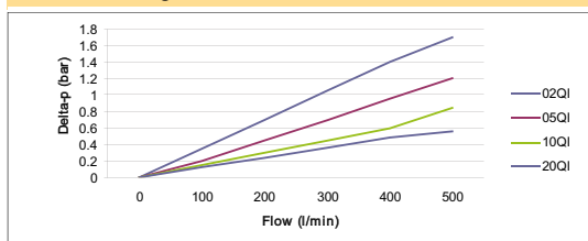
EPF Size 4 Length 2 Filter Elements
