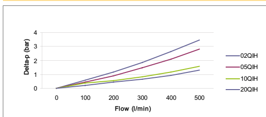
EPF Size 4 Length 1 High Strength Filter Elements
