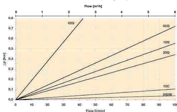
GA1-60 elements (Length 2)
