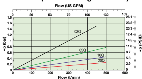
IN390 (3)(Element length code 11)
