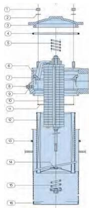
BGT-4 (conventional element)
