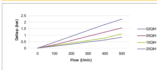
EPF Size 4 Length 2 High Strength Filter Elements
