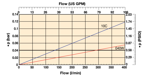
STF300 (Element length code 8)
