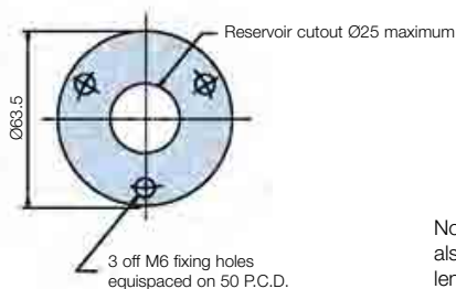
Pressurised spin-on air breather stem
