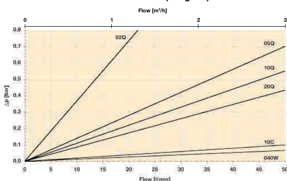
GA1-30 elements (Length 0)
