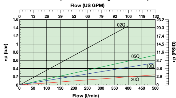
STF500 (Element length code 10)
