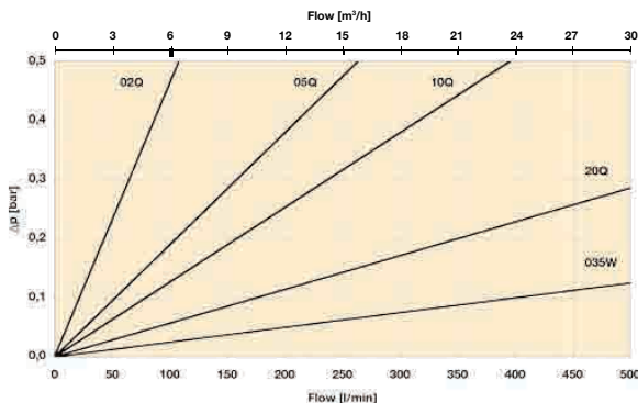
Elements for GS7
