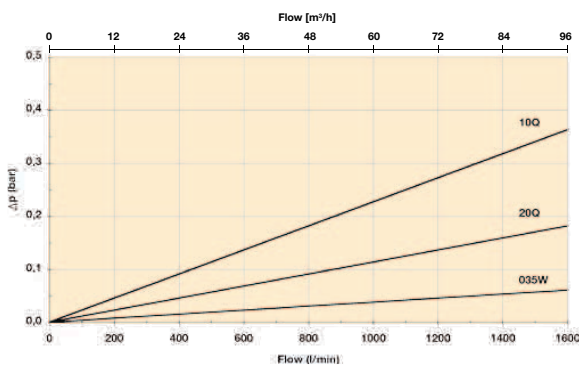
Length 3 element pack/both sides
