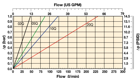
ETF90 (Element length code 3)
