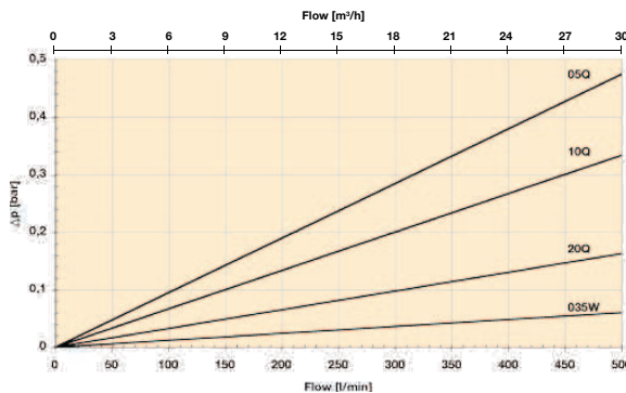
DF2089 elements/both sides
