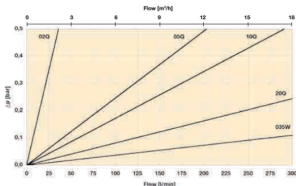
Elements for GS6
