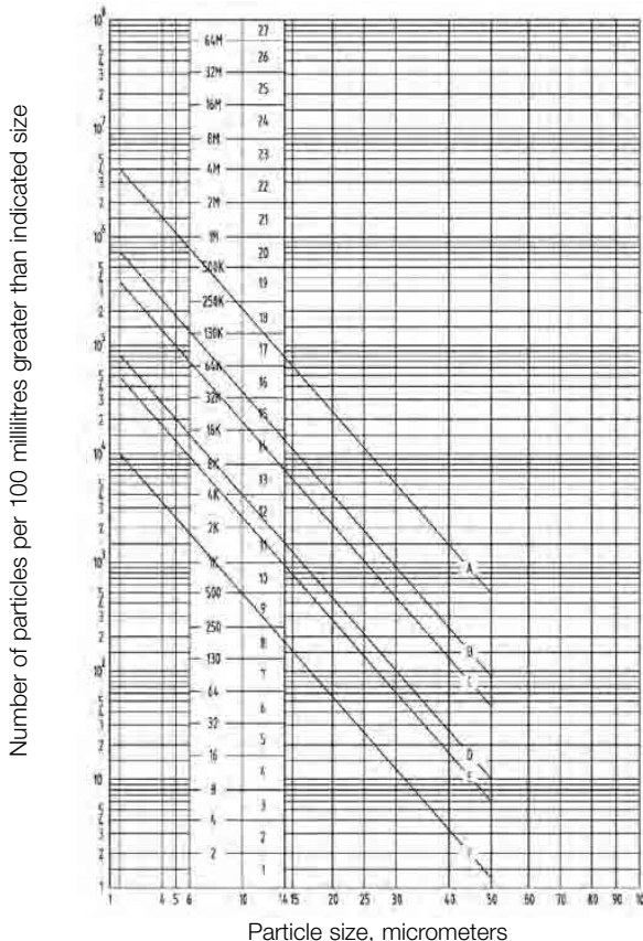
ISO 4406:1999 cleanliness classes
