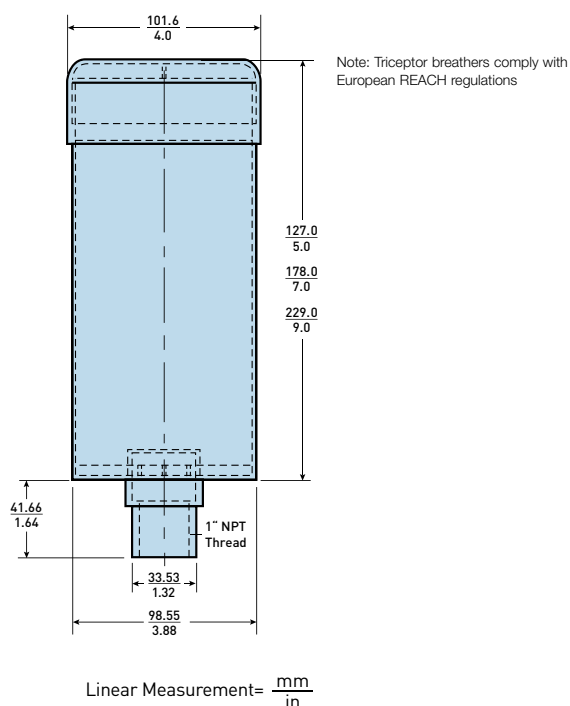
Field Adapter
