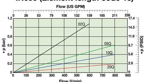
IN1000 (Element length code 15)
