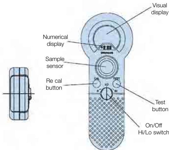
Function buttons
