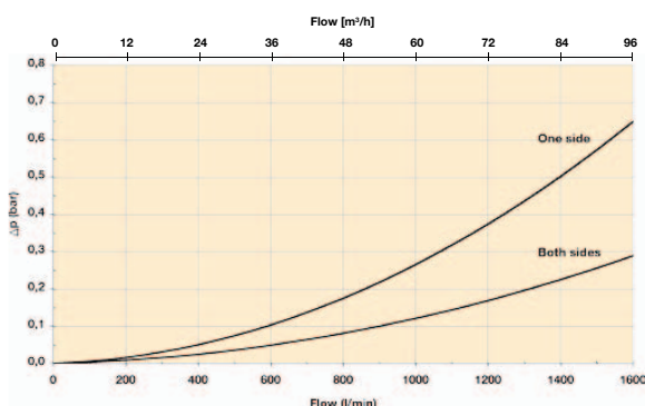
Length 2 element pack/one side
