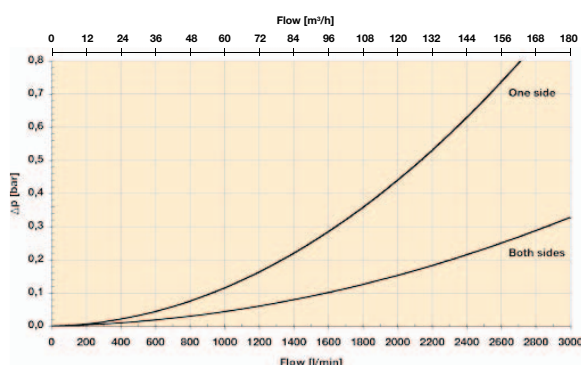
Length 2 element pack (2 pcs)/one side in use
