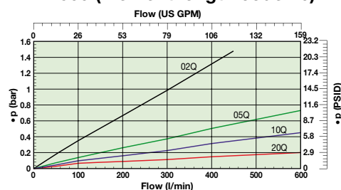
IN500 (3) (Element length code 12)
