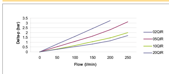
EPF Size 3 Length 1 Filter Elements with reverse flow valve
