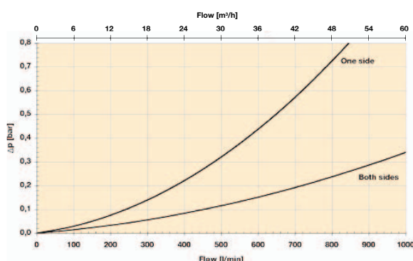
Length 2 element pack (2 pcs)/one side in use
