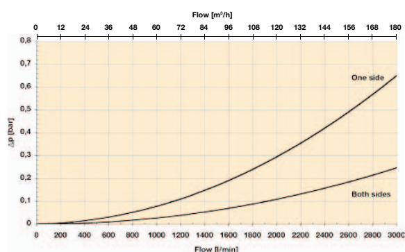
DFH2060 element pack (3 pcs)/one side in use
