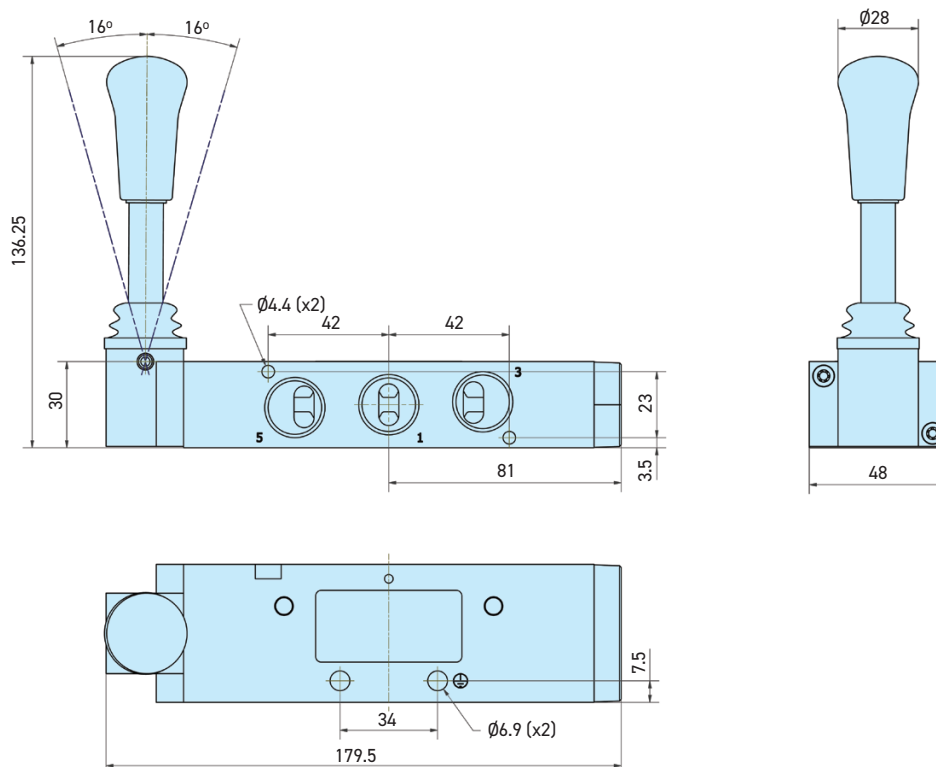
P2LDX - 5/3 Lever operated directional control valves
