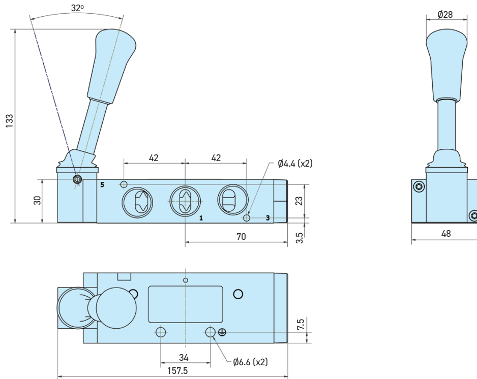
P2LDX - 5/3 Lever operated directional control valves
