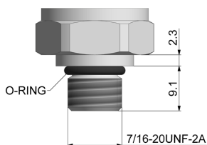
7/16-20UNF-2A
