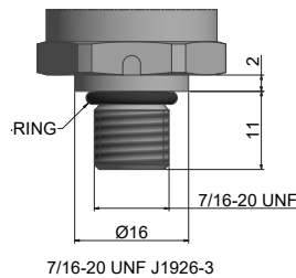
7/16-20 UNF J1926-3
