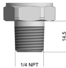
1/4"-18 NPT
