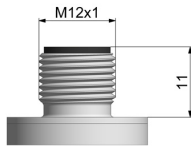
M12x1 Metallic
