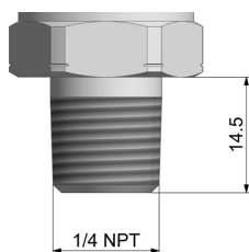
1/4"-18 NPT
