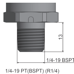
1/4-19 PT(BSPT) (R1/4)
