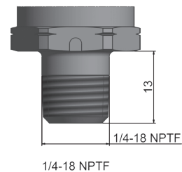
1/4-18 NPTF
