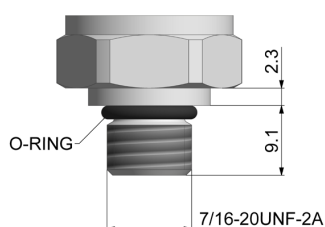
7/16-20UNF-2A
