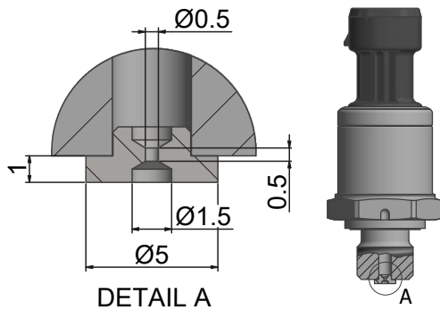
7/16-20 UNF J1926-3
