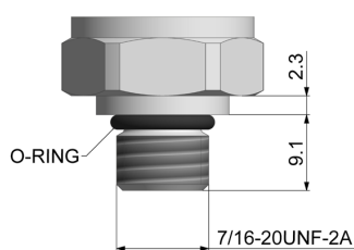
7/16-20UNF-2A
