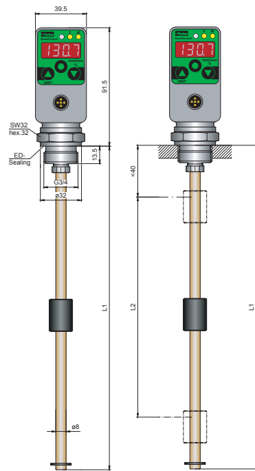
L1 = length of the sensor (mm) L2 = active range (mm)
