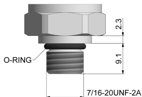
7/16-20UNF-2A
