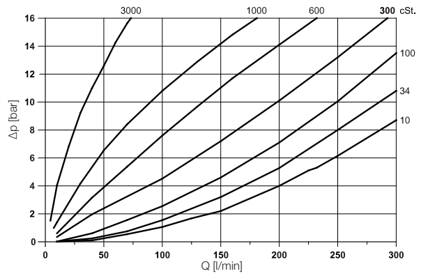
SCVF-300 \Delta p - Viscosity
