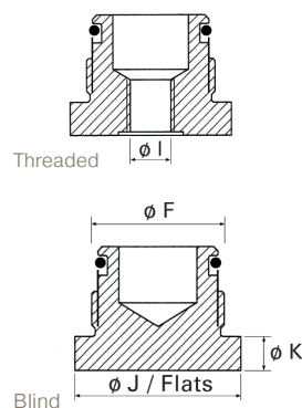
Shape B - Seal in fluid port
