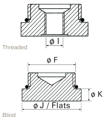
Shape A - Seal in angle
