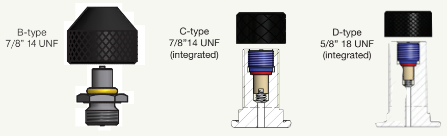
Model of valve stem
