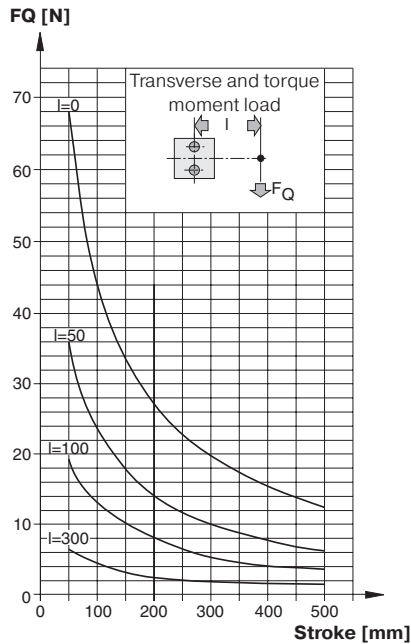
Transverse and Torque Moment Load - Ø 50 mm
