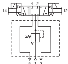
Common Port Regulator with 5/3 Closed Center
