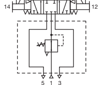
Common Port Regulator with 5/3 Closed Center
