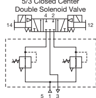
Independent Dual Port Regulator with 5/3 Closed Center
