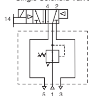
Common Port Regulator with 5/2 Single Solenoid Valve
