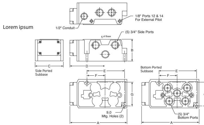
PS4211 Subbase Dimensions [mm]
