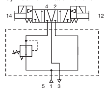
Independent Port Regulator with 5/3 Cylinder to Exhaust Function
