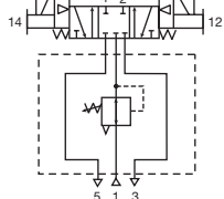
Common Port Regulator with 5/3 Closed Center
