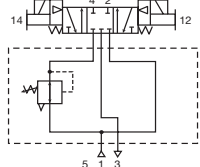
Independent Port Regulator with 5/3 Inlet to Cylinder Function
