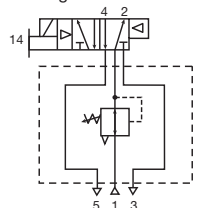
Common Port Regulator with 5/3 Closed Center
