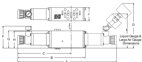
H1 Series Sandwich Regulator, Dimensions [mm]
