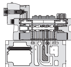
H1 5599-2 Single Solenoid Internal Pilot Manifold Mounted
