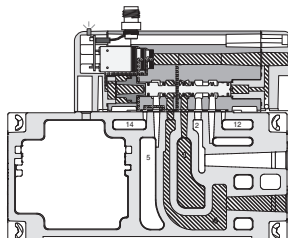
15407-1 18mm Single Solenoid Internal Pilot Manifold Mounted
