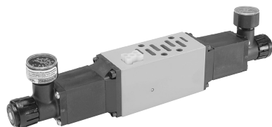
H1 - Size 1 (Independent Dual Port Regulator shown)
