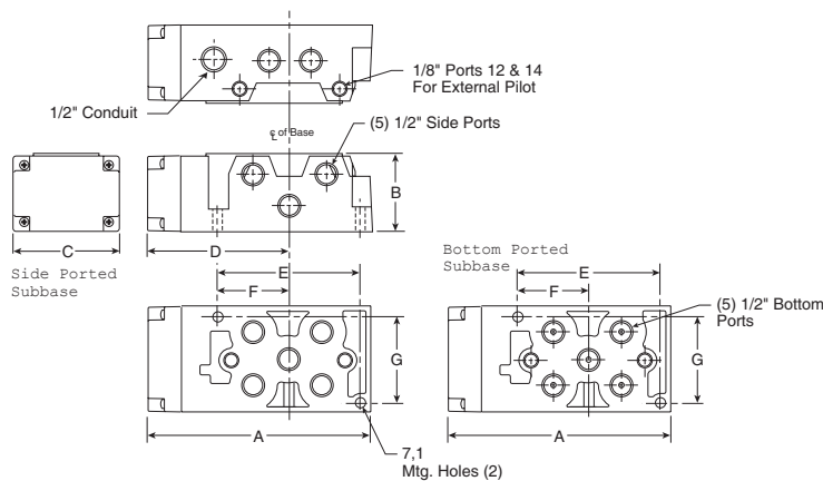
PS4111 Subbase Dimensions [mm]
