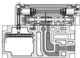
15407-2 26mm Double Solenoid External Pilot Manifold Mounted
