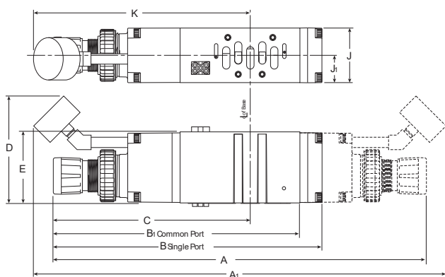
H2 & H3 Series Sandwich Regulator, Dimensions [mm]
