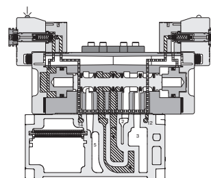
H2 5599-2 Double Solenoid External Pilot Manifold Mounted
