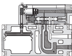
15407-2 18mm Single Solenoid Internal Pilot Manifold Mounted
