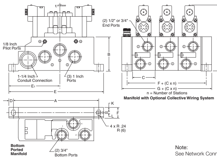
PS4211 Manifold Dimensions [mm]
