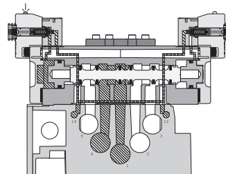
H3 5599-2 Double Solenoid External Pilot Subbase Mounted
