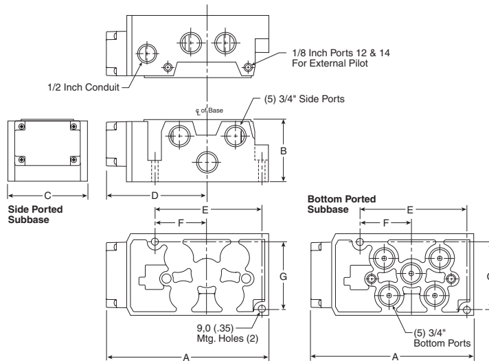
PS4211 Subbase Dimensions [mm]
