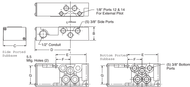
PS4011 Subbase Dimensions [mm]
