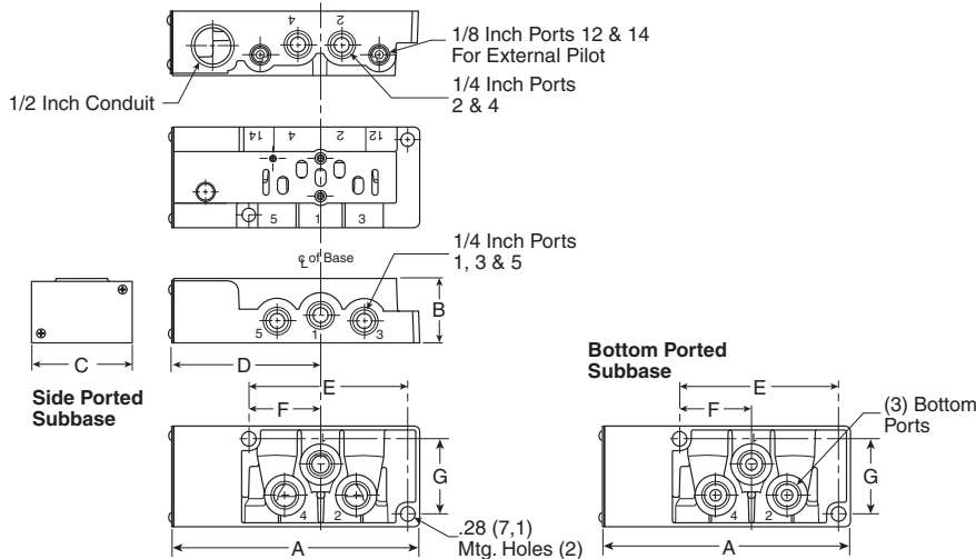
HA Dimensions [mm]
