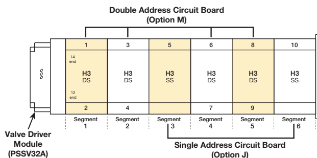
H3 Example - Six Segment Manifold Example
