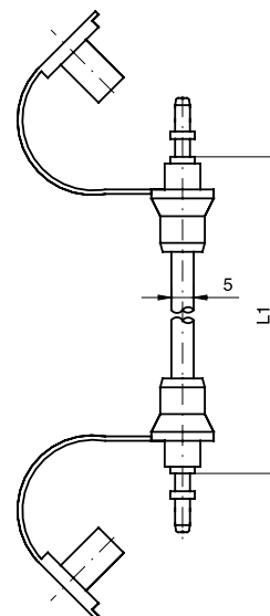
Test hose: SMA1
