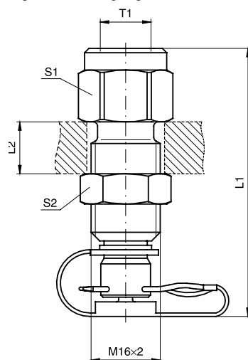
Pressure gauge connector: MAV-MA1
