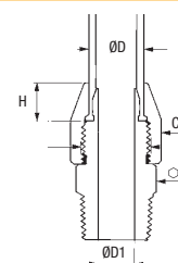
PL Nickel-Plated Brass Spigot Fittings
