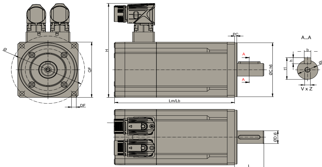
Dimensions [mm]
