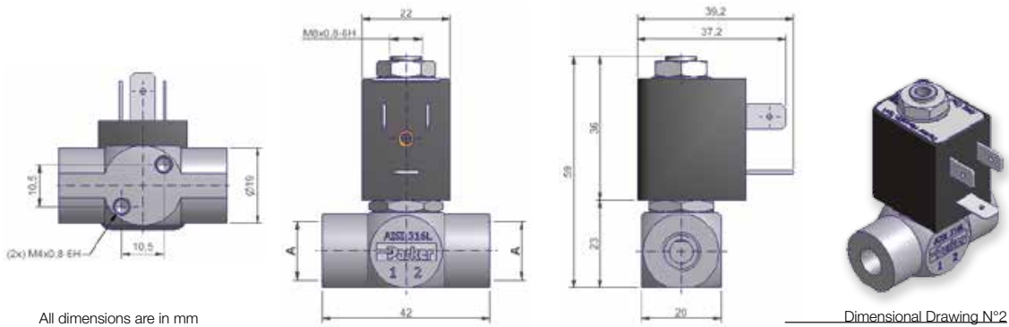
All dimensions are in mm
