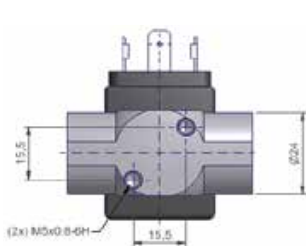
All dimensions are in mm
