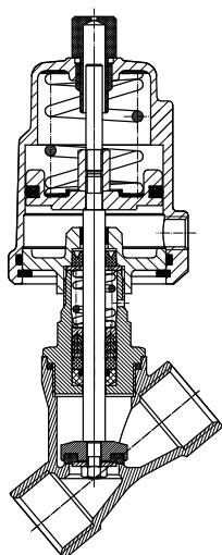
Normally Closed Valve
