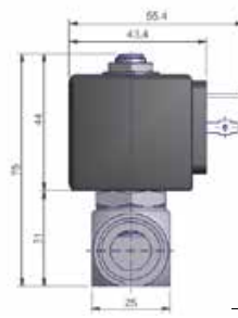
Dimensional Drawing N°2
