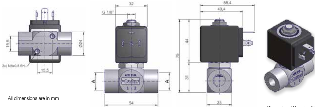
Dimensional Drawing N°1
