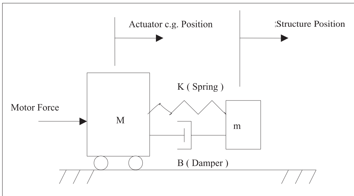
Schematic Diagram
