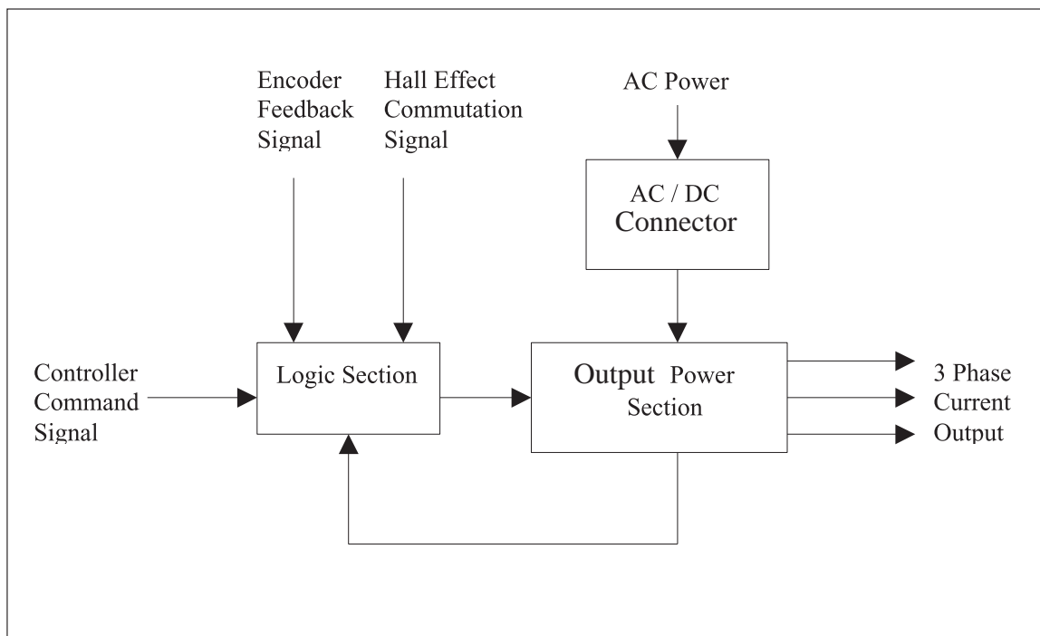
Block Diagram of a Typical Servo Amplifier
