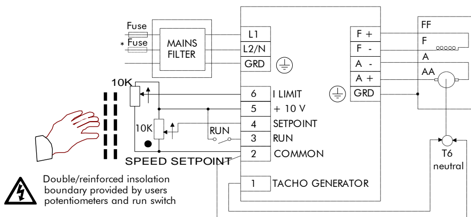
Figure 4.2 Wiring Diagram Current Control
