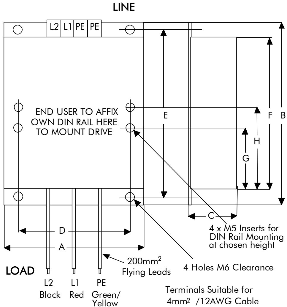
Figure 4.4 Filter Mechanical Arrangement
