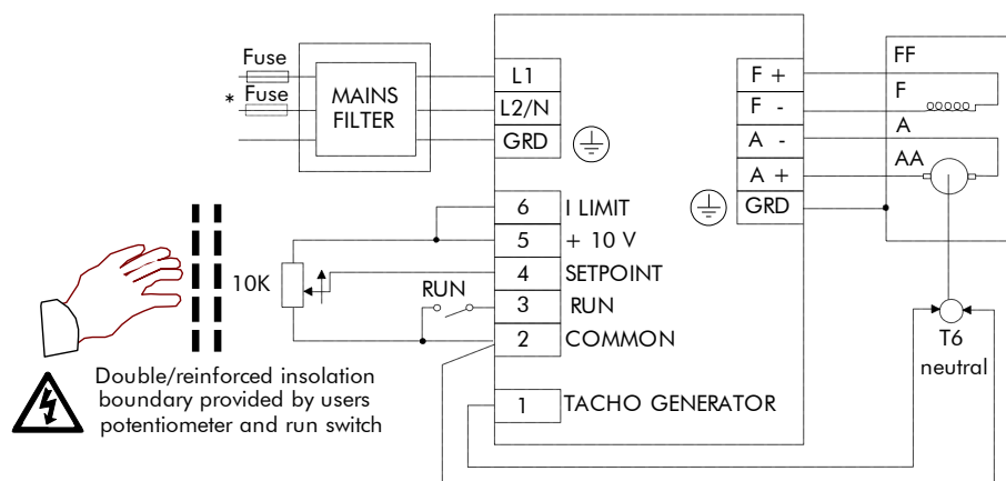
Figure 4.1 Wiring Diagram Speed Control
