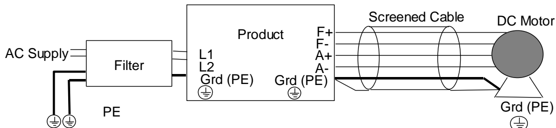
Figure 4.5 Wiring Diagram Mains Filter
