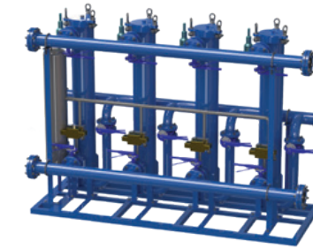
Series BPS 14 14 Barrels/Minute Manual System
