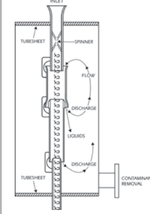
Series 95V-CT Separator
