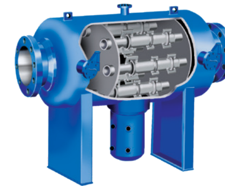
Series 95H-CT Separator
