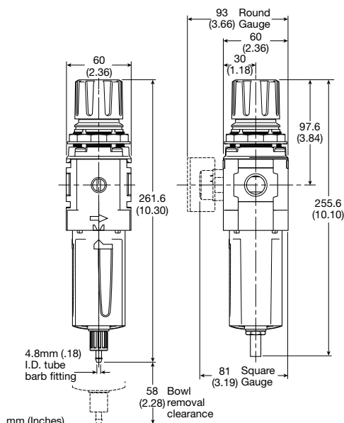
Manual Drain
