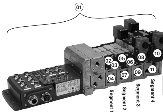
Example: 5 segment manifold with (2) HB, (2) HA, (1) H1, and (1) H2 valve on manifold bases with PCH Network Portal end plate.
