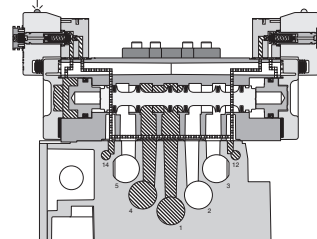
H3 5599-2: Double Solenoid External Pilot Subbase Mounted
