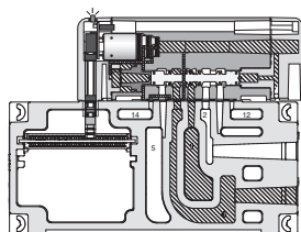
15407-2: 18mm Single Solenoid Internal Pilot Manifold Mounted
