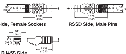
RJ45S Side
