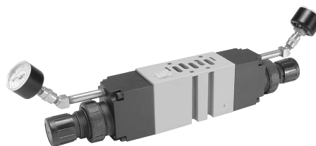
H2 - Size 2 (Independent Dual Port Regulator shown)
