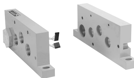
H3 25-pin D-Sub end plate shown
