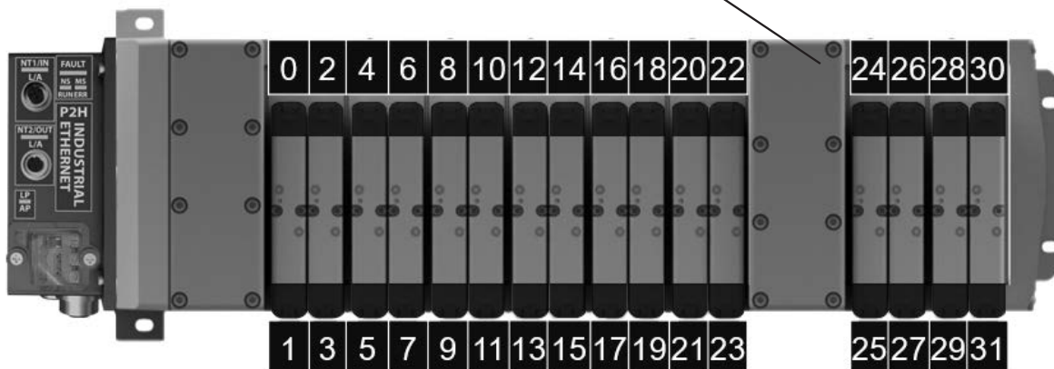
Intermediate air supply module shown
