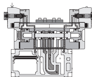
H2 5599-2: Double Solenoid External Pilot Manifold Mounted
