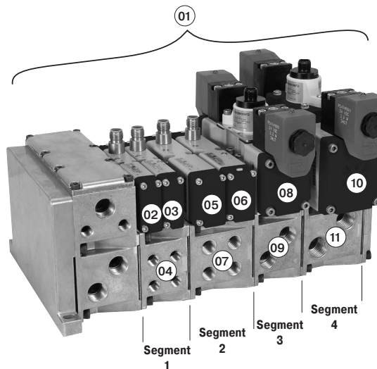
Example: 4 segment manifold with (2) HB, (2) HA, (1) H1, and (1) H2 valve on manifold bases with low profile, NPT end plate.
