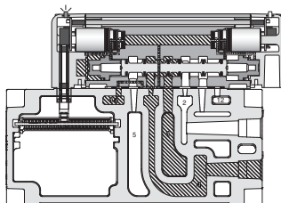
15407-2: 26mm Double Solenoid External Pilot Manifold Mounted
