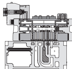
H1 5599-2: Single Solenoid Internal Pilot Manifold Mounted
