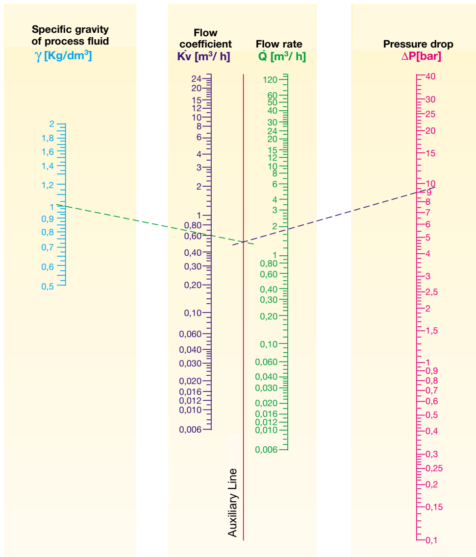
Diagram 1 for liquids (up to 3°E)
