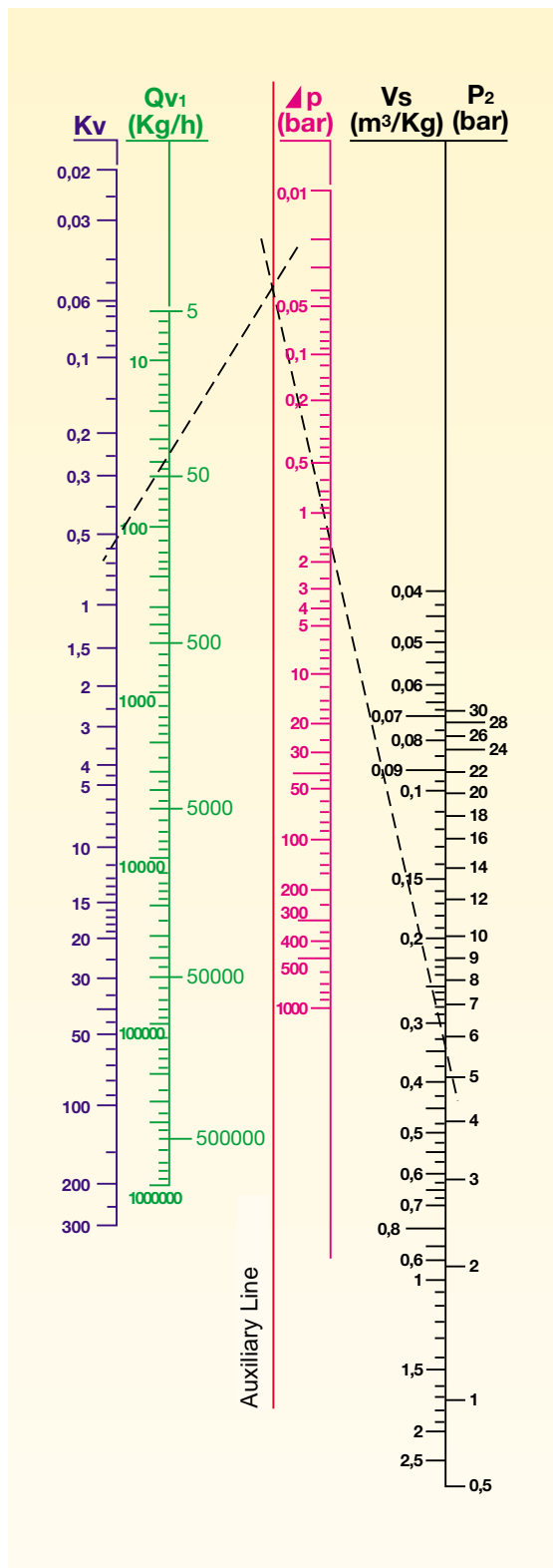
Diagram 3 for dry saturated steam
