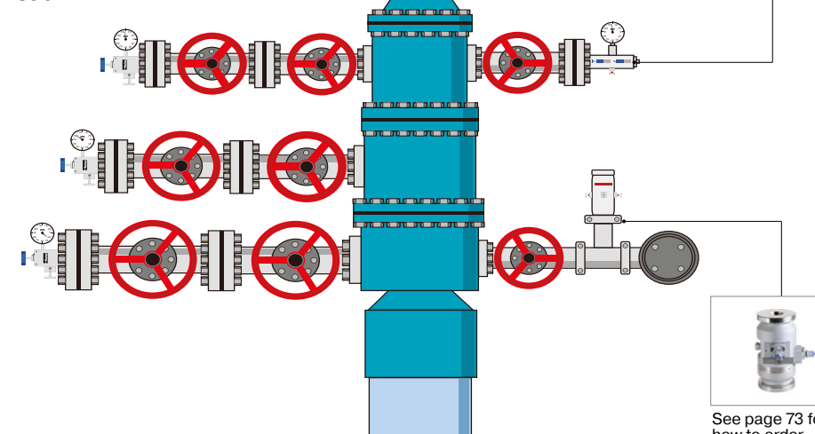
Wellhead
