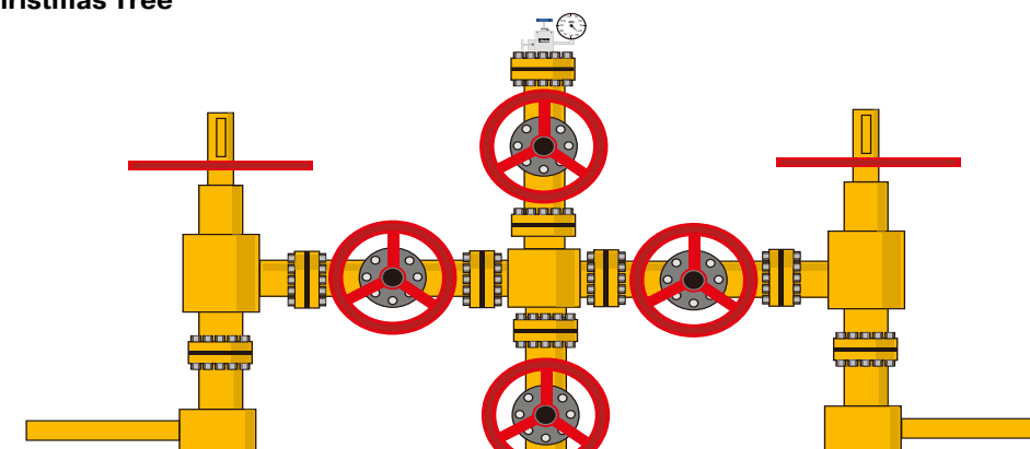
Christmas Tree
