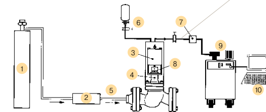
Prototype testing schematic as per ISO 15848-1
