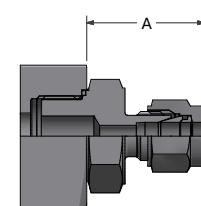
PTFree connect™ male connector (Code PFC)
