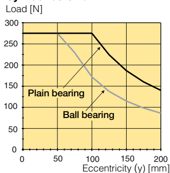
Cylinder bore 50 mm
