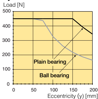
Cylinder bore 100 mm
