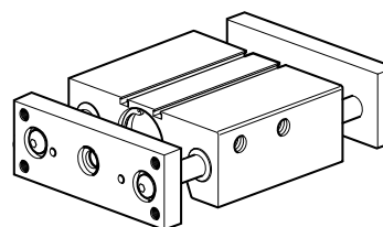
Double acting with two fixing plates, side connections are recommended.
