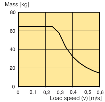
Cylinder bore 50 mm
