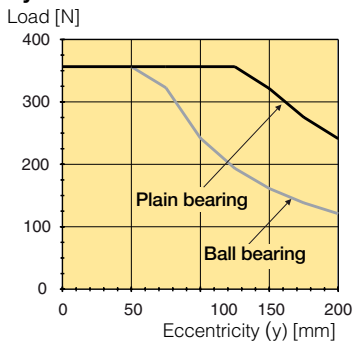
Cylinder bore 80 mm
