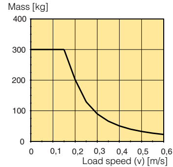
Cylinder bore 100 mm
