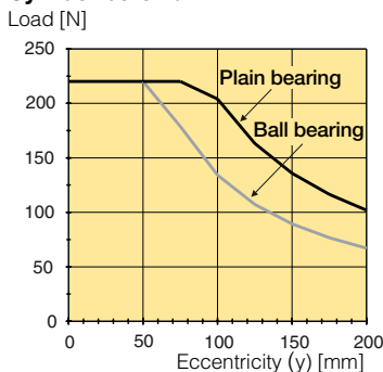
Cylinder bore 40 mm
