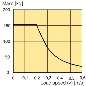
Cylinder bore 63 mm
