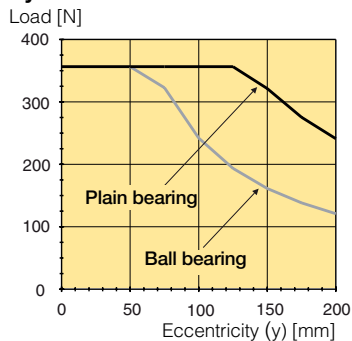
Cylinder bore 63 mm
