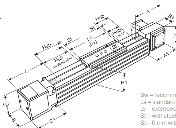
LBB with toothed belt without steel strip cover
