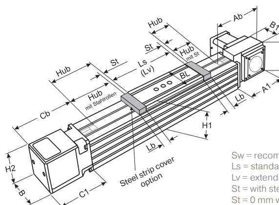
LBB with toothed belt and steel strip cover
