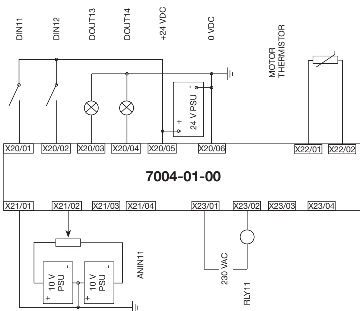
Example connection details for 7004-01-00 GPIO module
