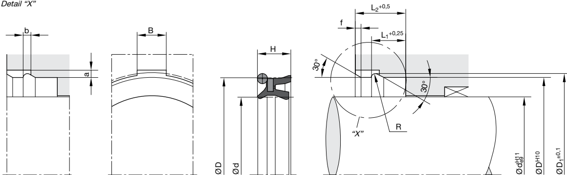
Detail "X"
