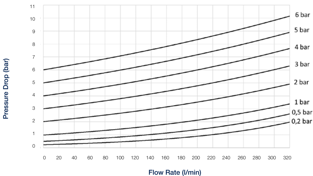
Pressure Drop Tube O.D. 35+42L/38S; size 24; female BSPP 11/2; RVP 55; DN 29
