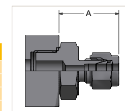
PTFree connect™ male connector (Code PFC)
