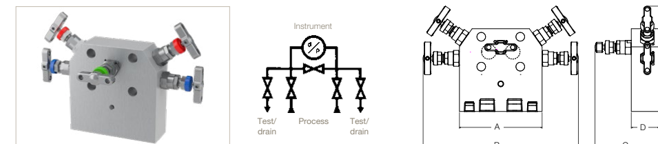
HD*5MCPEXT - Female threaded - NPT x Flanged
