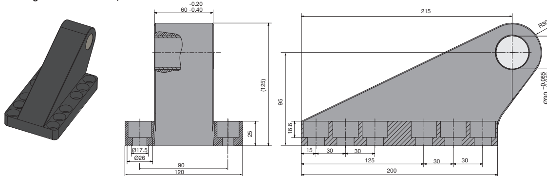
Bearing block for ETH125, Part No. 0152.039
