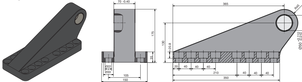
Bearing block for ETH125, Part No. 0152.039
