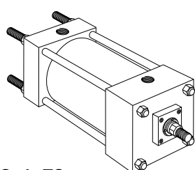
Style TC Tie Rods Extended Cap End (NFFA Style MX2)
