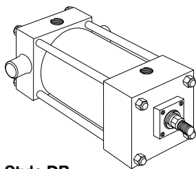
Style DB Cap Trunnion (NFPA Style MT2)
