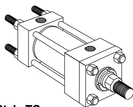
Style TC Tie Rods Extended Cap End (NFA Style MX2)
