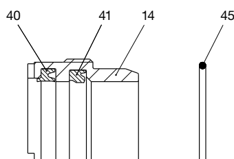
2AN Gland Cartridge and Seals
