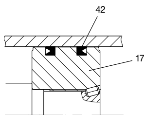
Lipseal Piston
