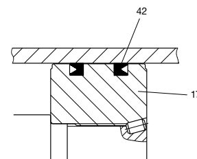
Lipseal Piston
