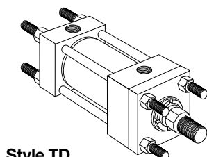
Style TD Tie Rods Extended Both Ends (NFA Style MX1)
