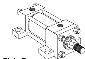
Style C Side Lug Mounting (NFA Style MS2)
