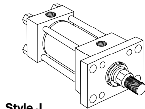
Style J Head Rectangular Flange (NFA Style MF1)
