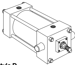
Style D Head Trunnion (NFPA Style MT1)
