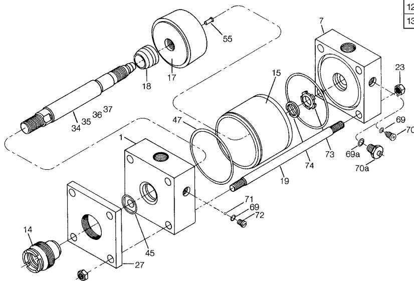
Lipseal Piston
